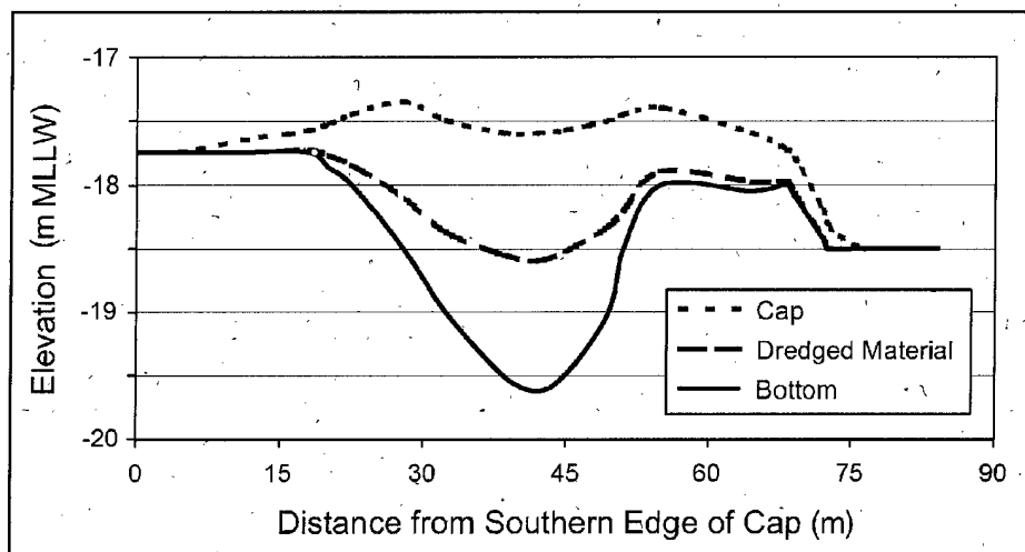
Figure 1. Representative cross section of the Duwamish Disposal Area with cap
