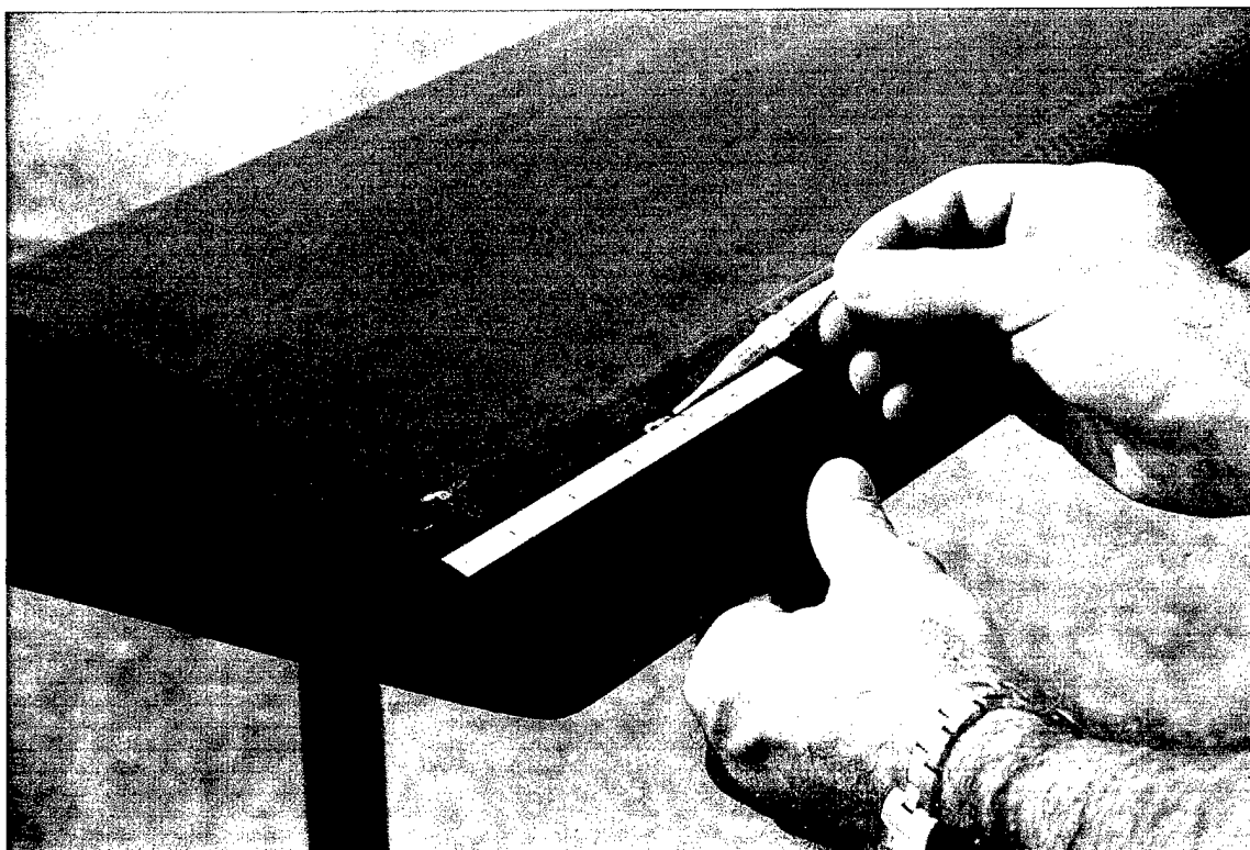
Figure 5.4. Dimpletape® Debond Position and Length.
