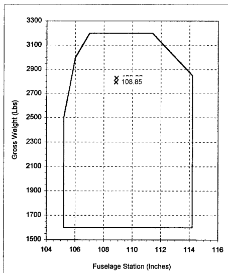
Figure C.14. Weight and Balance Hover 10% Optimum Dimpletape Length - Moved 2" Fwd - Light
