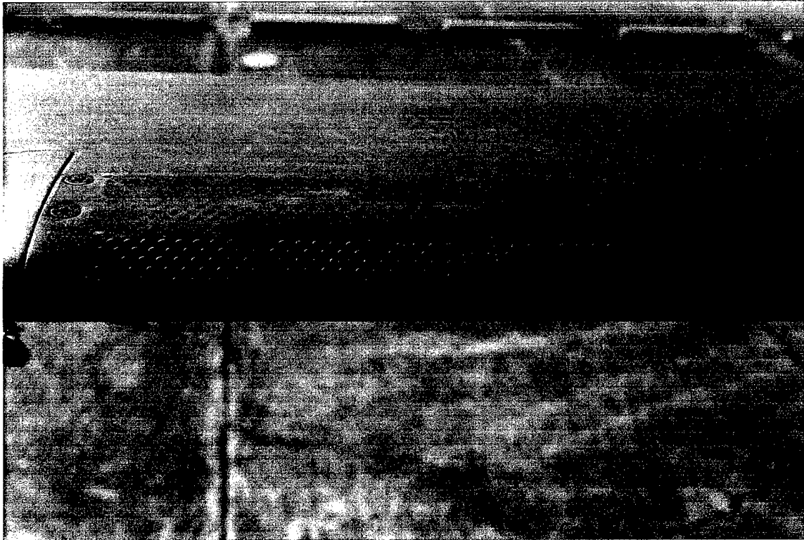
Figure 5.8. Dimpletape® Moved Forward Cordwise Two Inches from Maximum Camber Point.
