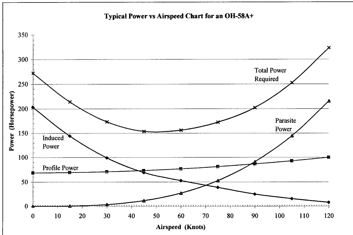
Figure 5.1. Components of Power Required in Level Flight.
