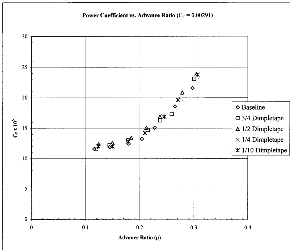
Figure B.10. Power Coefficient versus Main Rotor Blade Advance Ratio,
