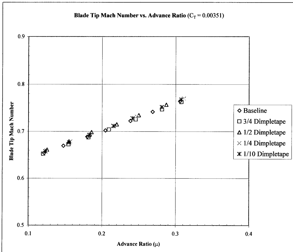
Figure B.13. Blade Tip Mach Number versus Main Rotor Blade Advance Ratio, C T = 0.00351.
