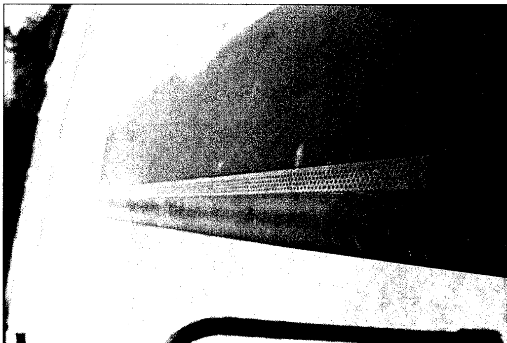
Figure E.8. Overhead Dimpletape® View (50% Rotor Blade Length).
