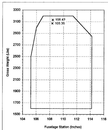
Figure C.13. Weight and Balance Hover 10% Optimum Dimpletape Length - Moved 2" Fwd - Heavy
