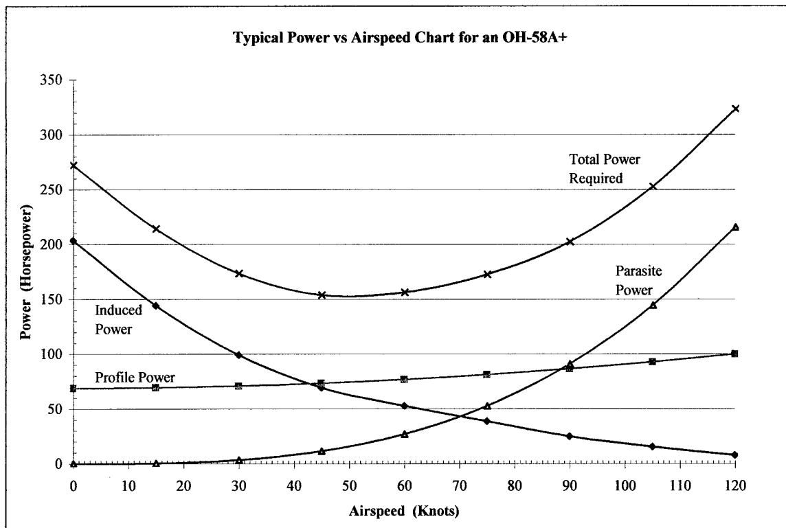
Figure 2.1. Components of Power Required in Level Flight.
