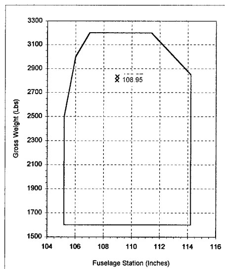
Figure C.12. Weight and Balance Hover 10% Optimum Dimpletape Length - Moved 1" Fwd - Light
