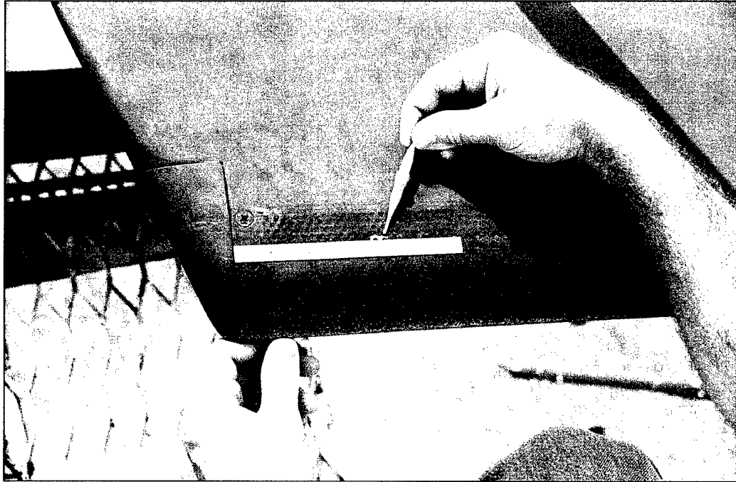
Figure E.2. Dimpletape® Debond Repair.
