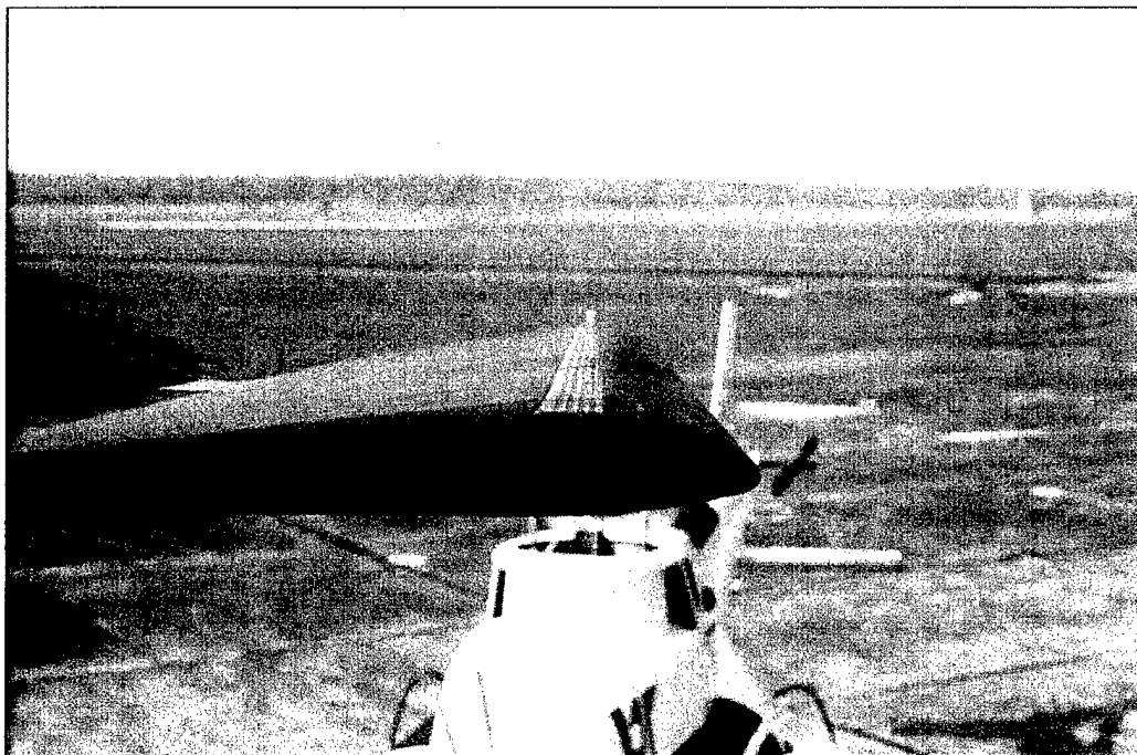
Figure E.7. Initial Maximum Camber Dimpletape® Positioning.
