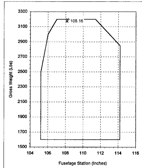
Figure C.15. Weight and Balance Hover 10% Optimum Dimpletape Length - Moved 1" Aft - Heavy
