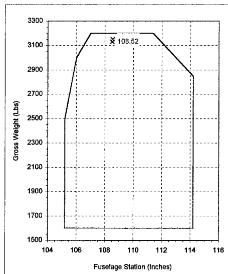
Figure C.11. Weight and Balance Hover 10% Optimum Dimpletape Length - Moved 1" Fwd - Heavy
