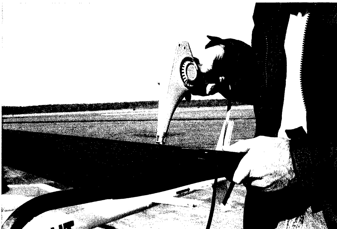
Figure E.15. Heating Rotor Blade with Hot Air Gun Prior to Dimpletape® Application.
