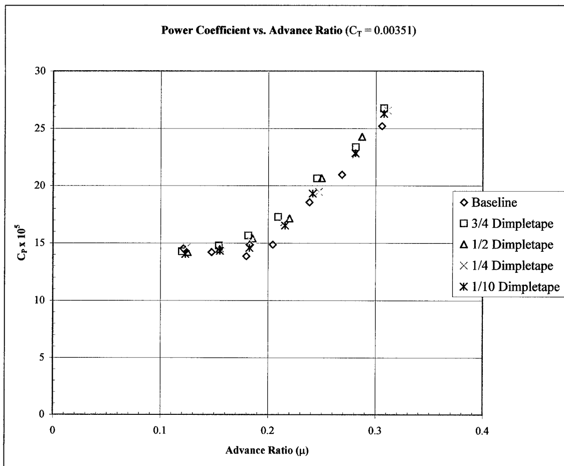
Figure B.11. Power Coefficient versus Main Rotor Blade Advance Ratio, C T = 0.00351.
