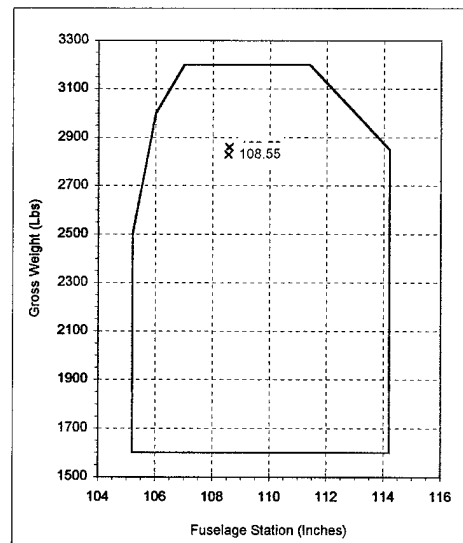
Figure C.16. Weight and Balance Hover 10% Optimum Dimpletape Length - Moved 1" Aft - Light
