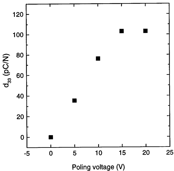
Figure 12c. d_{33} increases with increasing poling field and reaches a saturation value of 103 pC/N at a poling field of about 3E_c .
