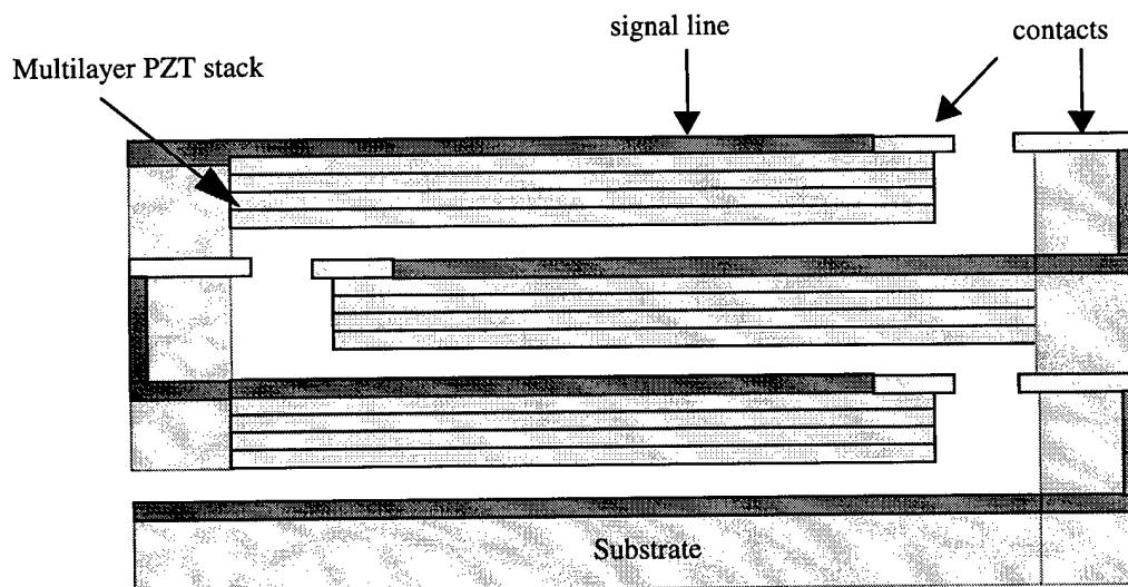
Figure 24. Series switch with stacked PZT layers
