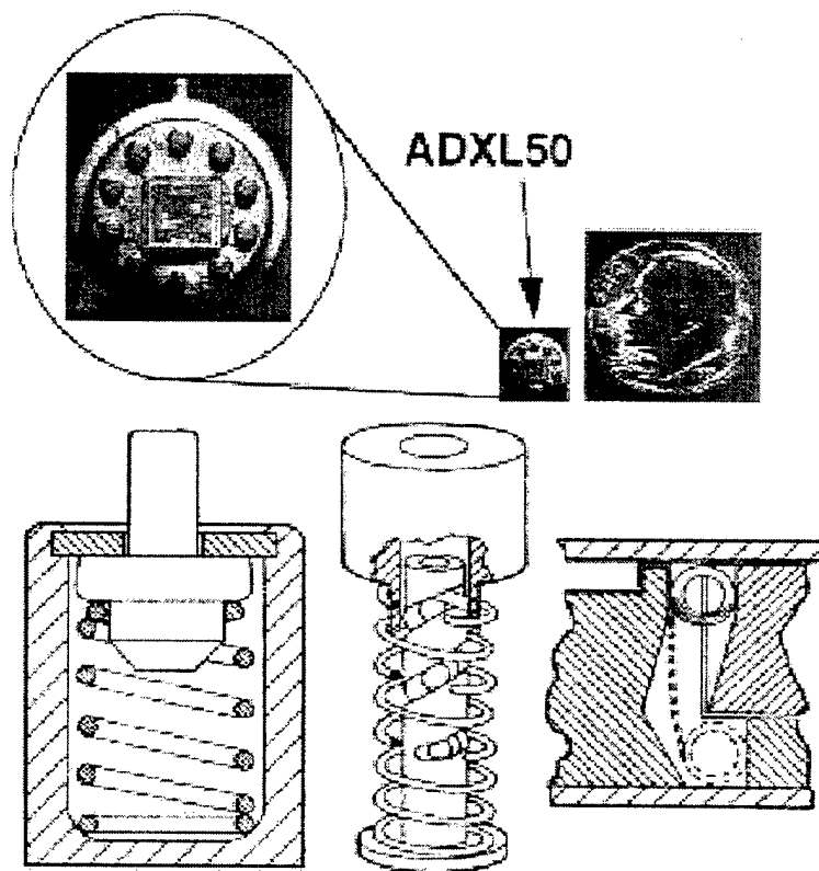
FIGURE 11. ADXL50 FUZE SAFE-ARM DEVICE
