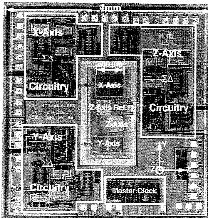
FIGURE 4. A THREE-AXIS ACCELEROMETER
