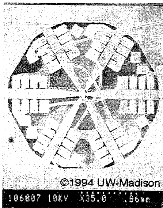
FIGURE 3. A THREE PHASE MAGNETIC MOTOR
