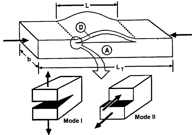
Figure 43. Composite Plate With an Interlaminar Defect. The Delamination Divides the Plate Into Two Parts: (D) the Buckled Sublaminates and (A) the Parent Laminate. At the Crack Tip, Both Normal and Shear Stress Develop Causing Mode I and Mode II Crack Displacements, Respectively (Gillespie and Carlsson 1991).
