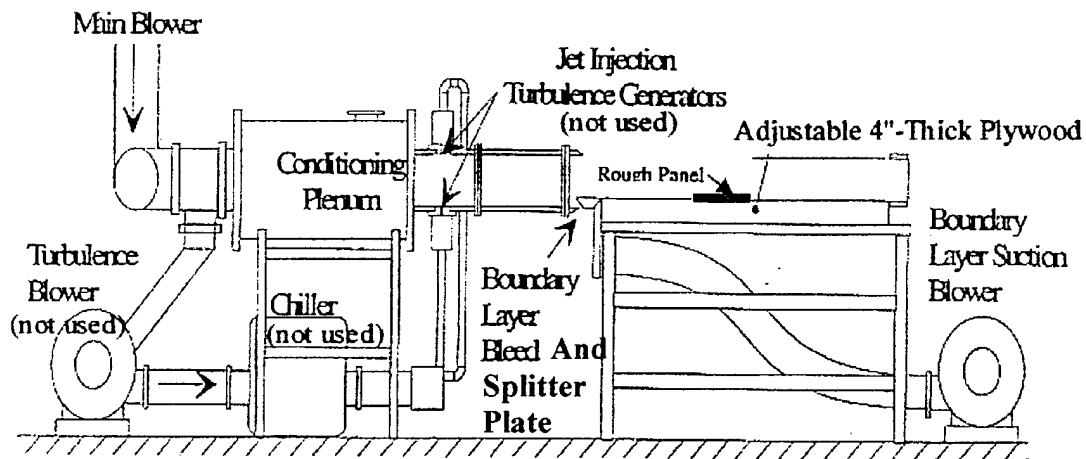
Figure 3.7 Boundary Layer Wind Tunnel Side View Schematic
