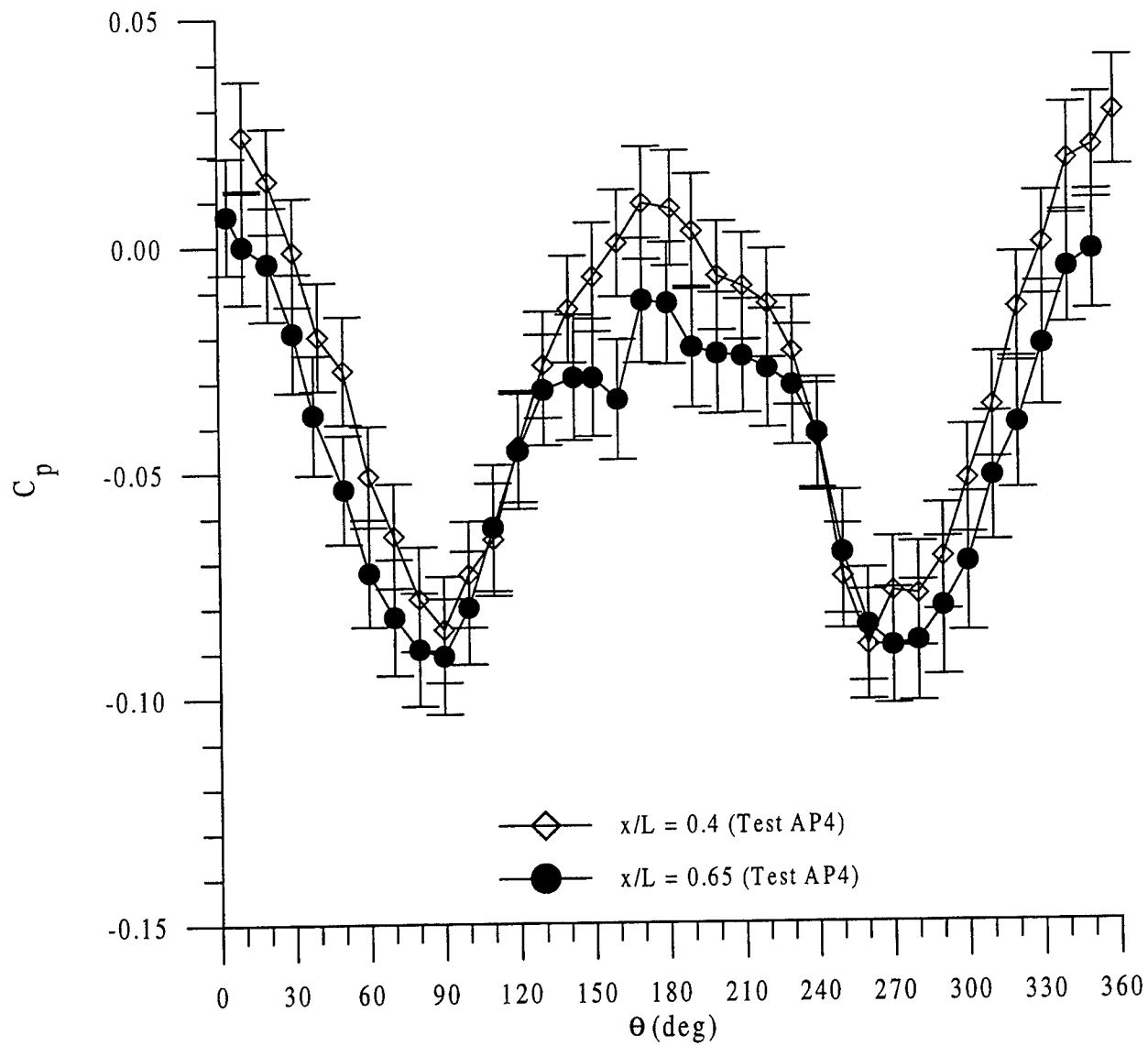
Figure 6 Circumferential pressure distributions: \beta = 9.5 deg, U = 7.64 m/s, sail off
