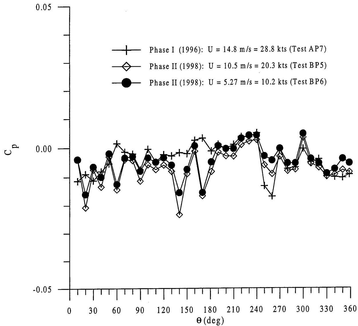
Figure 62 Comparison of Phase I and II pressure distributions: \beta = 0^\circ , sail off, x/L = 0.47
