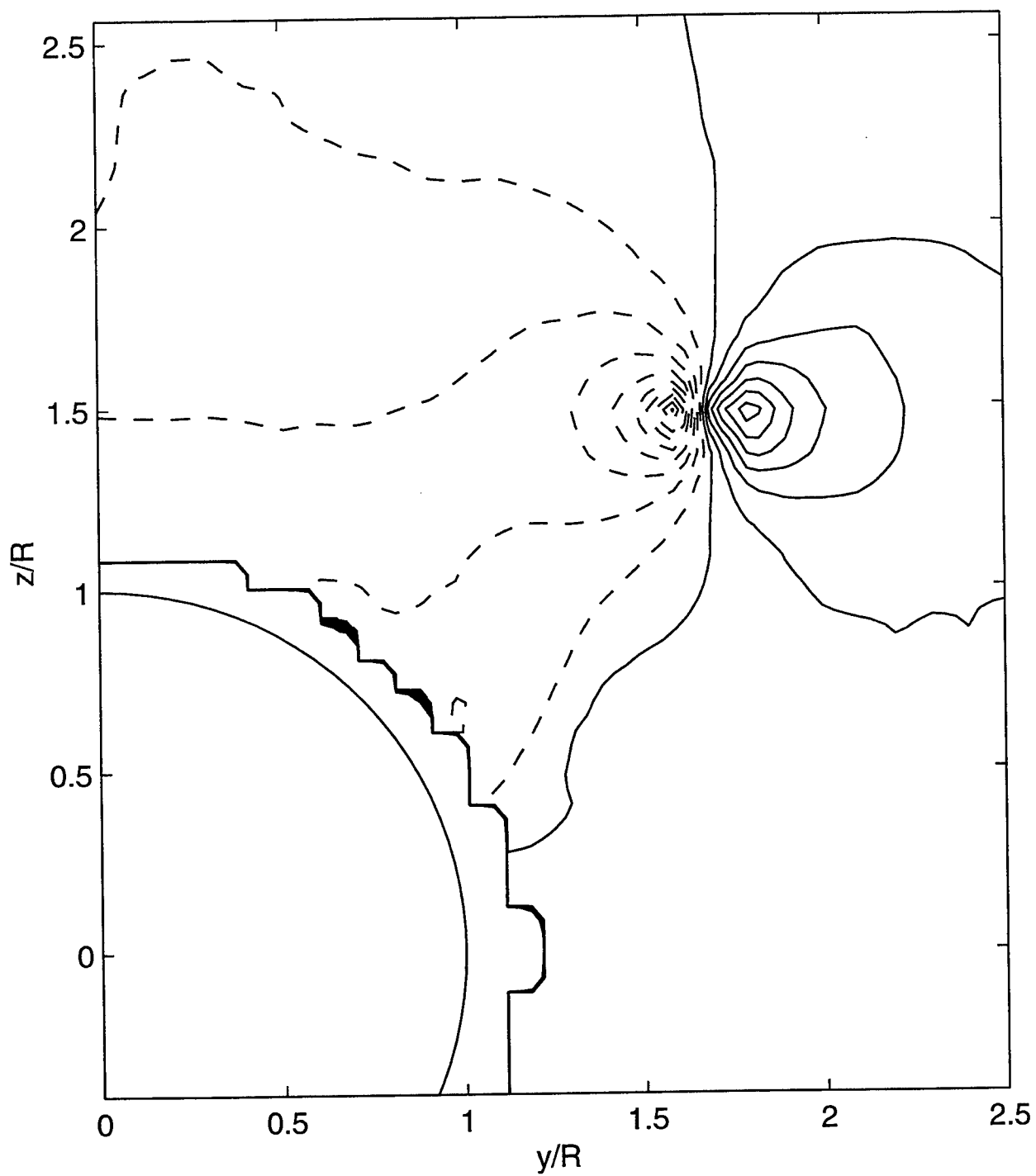
Figure 26 Transverse velocity contours: \beta = 9.5^\circ , U = 14.9 \text{ m/s} , sail on, x/L = 0.65 (Test AV08)
