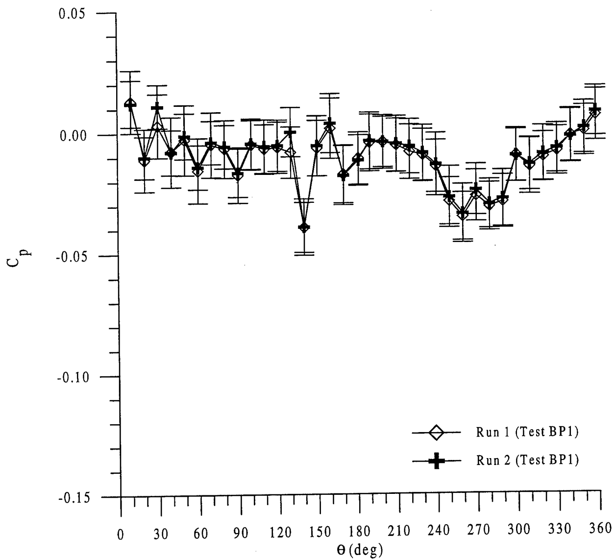
Figure 49 Circumferential pressure distributions: \beta = 5 deg, U = 9.18 m/s, sail on, x/L = 0.47
