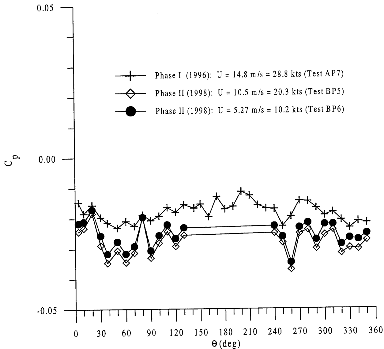
Figure 63 Comparison of Phase I and II pressure distributions: \beta = 0 deg, sail off, x/L = 0.65
