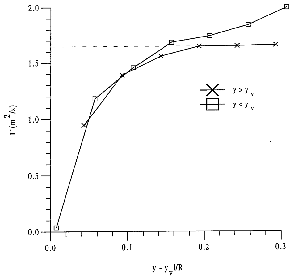
Figure 38 First estimate of vortex circulation using potential vortex: \beta = 9.5^\circ , U = 14.9 \text{ m/s} , x/L = 0.47
