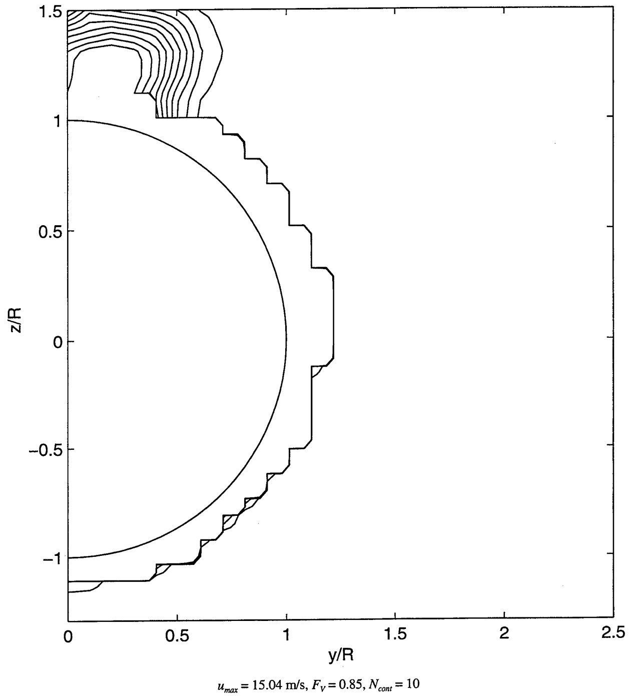
Figure 35 Streamwise velocity contours: \beta = 0 deg, U = 14.9 m/s, sail off, x/L = 0.47 (Test AV17)
