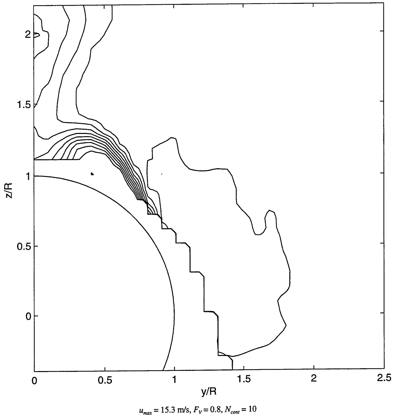
Figure 29 Streamwise velocity contours: \beta = 9.5 \text{ deg} , U = 14.9 \text{ m/s} , sail off, x/L = 0.65 (Test AV09)
