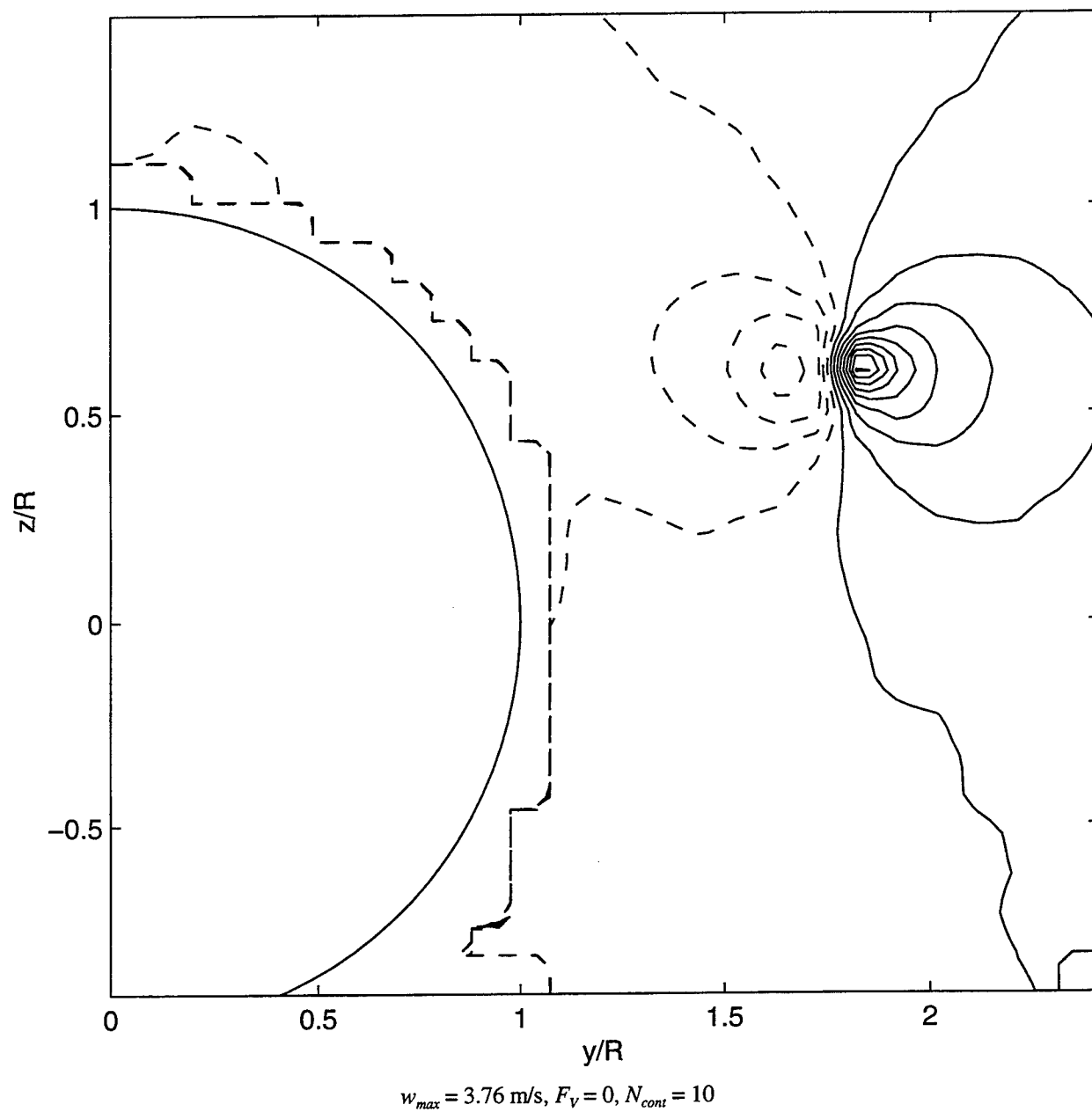
Figure 83 Transverse velocity contours: \beta = 9.5 deg, U = 5.23 m/s, sail on, x/L = 0.48 (Test BV08)
