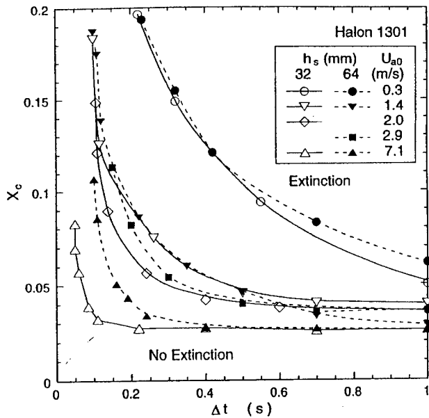
Fig. 3 The critical agent mole fraction at suppression vs. agent injection period.
