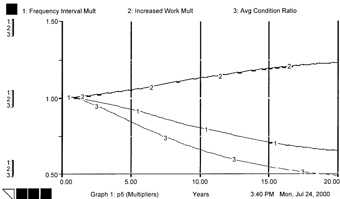
Figure 62. Average condition Impacts Workload
