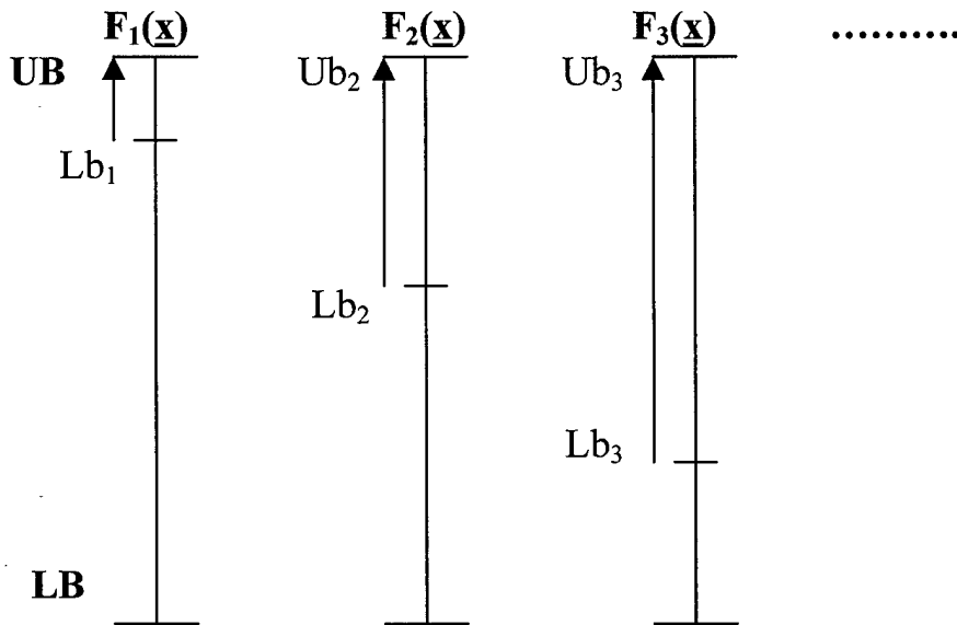
Figure 2.7 The Search Space for the 3-Objective Preemptive Goal Programming
