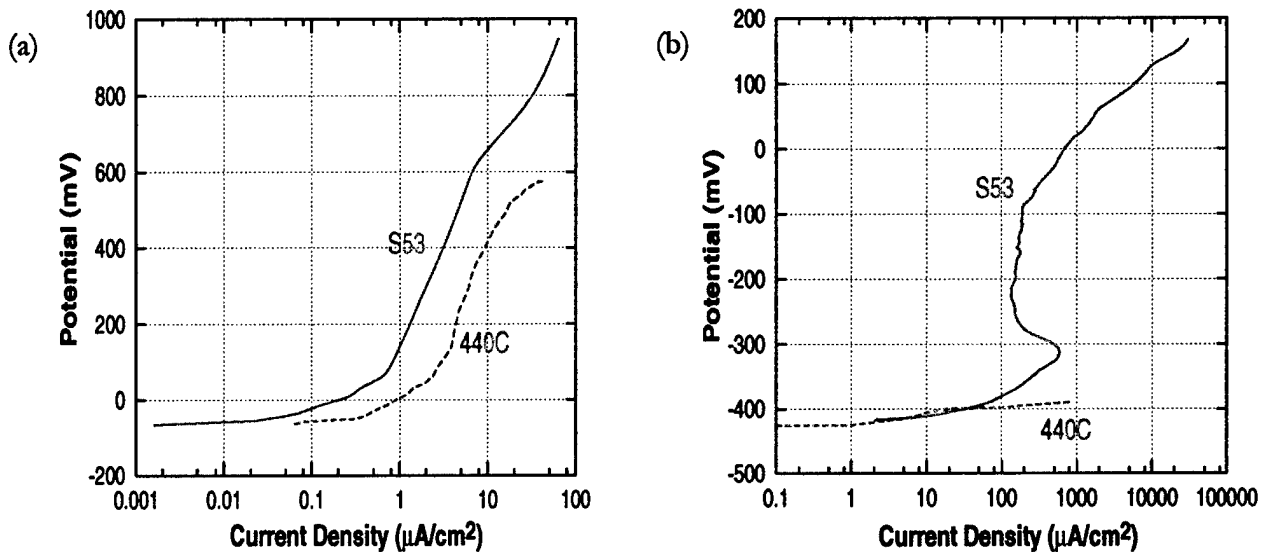
Figure 13. Anodic polarization curves of heat treated samples in (a) neutral water with 1% sucrose and (b) 3.5% NaCl as compared to 440C stainless steel.
