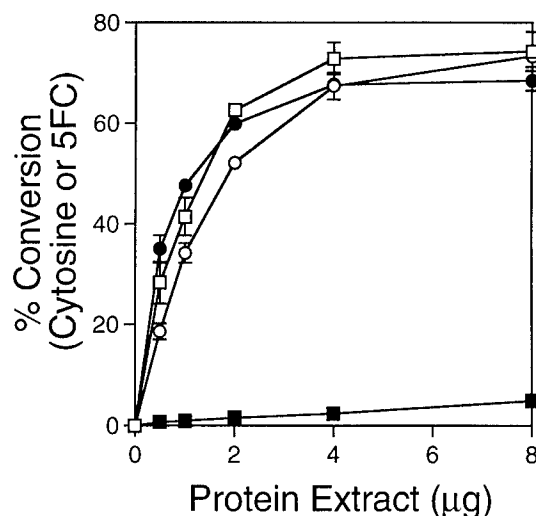
FIG. 2. YCD converts 5-FC to 5-FU more efficiently than BCD. Cell extracts from transiently transfected COS-1 cells were used to measure the conversion of 1 mM cytosine or 5-FC in 2 hr, as described in Materials and Methods. Conversion of cytosine by BCD (open squares) or YCD (open circles), and conversion of 5-FC by BCD (closed squares) and YCD (closed circles) are shown. Data represent the means and standard errors of four experiments.
