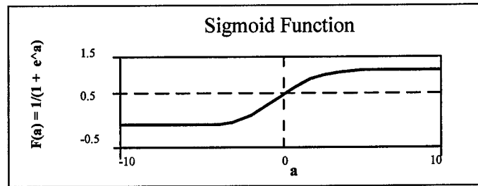
Figure 2-8. Sigmoid Activation Function.
