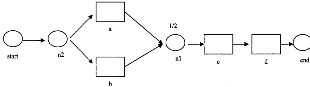
Figure 8. Simple System Built in RAPTOR.
