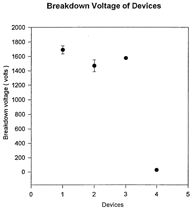
Fig. 12 Breakdown voltage of the devices (1) Low \text{H}^+ implanted devices (2) Two low \text{H}^+ implanted devices (3) High \text{H}^+ implanted devices (4) \text{He}^+ implanted devices
