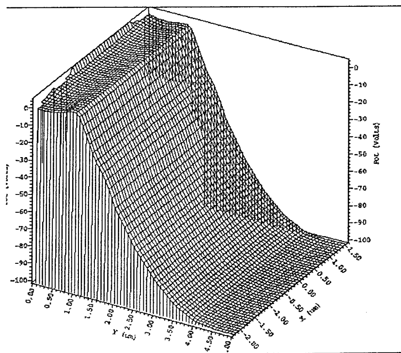
Fig. 8(a) Potential plot in the device at back contact potential of -100\text{V}
