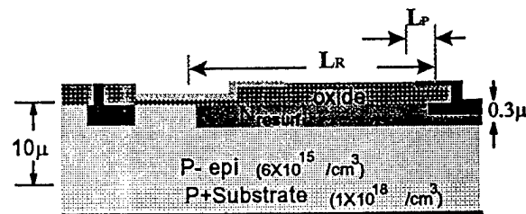
Lateral RESURF Inversion MOSFET
