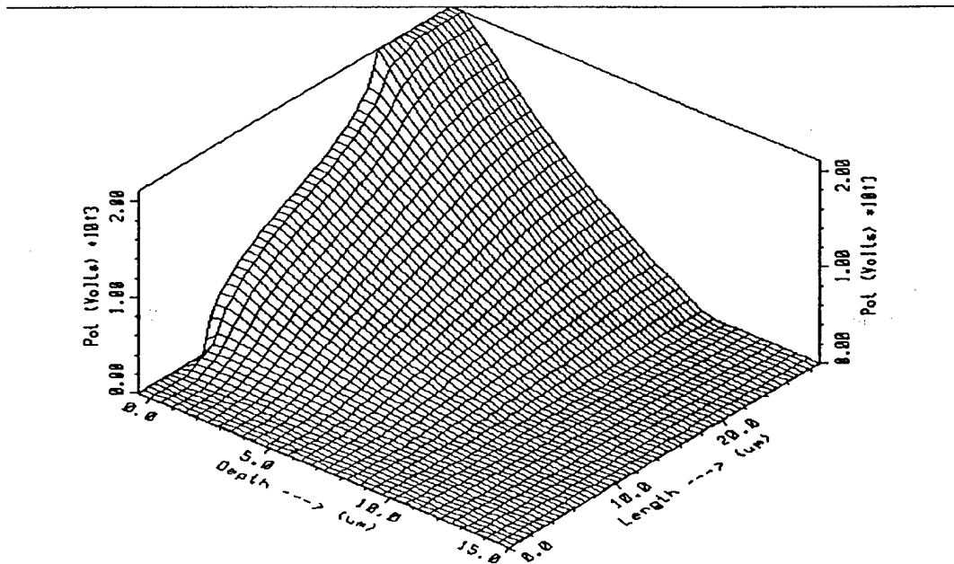
Fig 30 3-D Plot of the Potential distribution in the diode for a dose of 7 \times 10^{12} / \text{cm}^2
