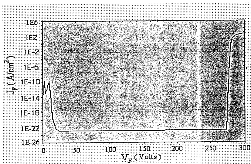
Fig. 5. J_F vs V_F for (a) Schottky diode (b) Schottky diode with isolation layer
