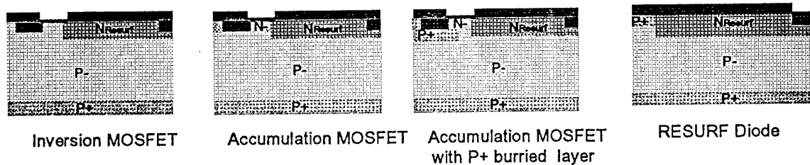
Figure 7. Cross-section of the devices after Gate oxide-deposition
