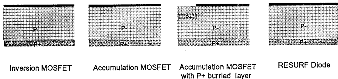
Figure 2. Cross-section of devices after P+ buried implants.
