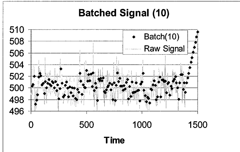
Figure 10. Batched Signal
