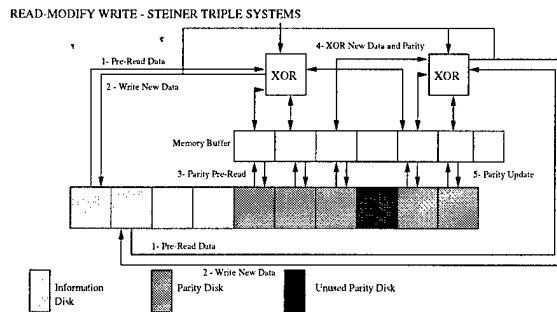
This is a scenario with 2 information disks in the same stripe that share one parity disk. Each of the information disks is first read and written. Next the needed parity disks are read and buffered in memory. Each parity in the buffer is XOR'ed with the old data and new data. The new information is written back to each of the parity disks.
