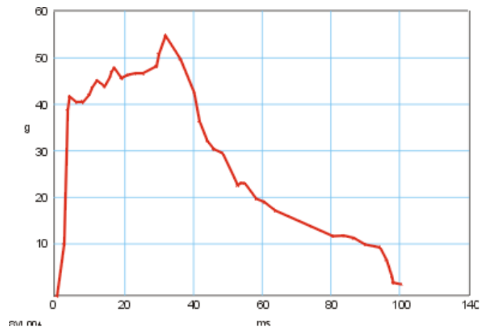
Figure 10 : Launch Accelerations
