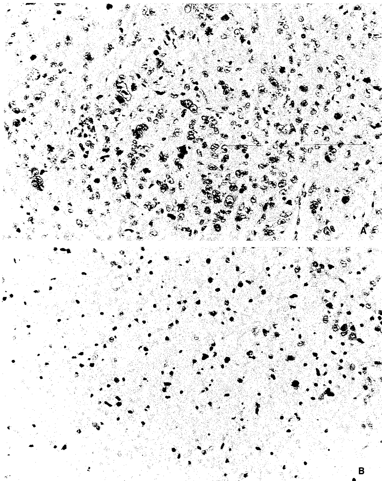
Figure 7. Tumor histology in mice treated with either compd E 1 or diluant control. (A) Control tumor showing infiltrating poorly differentiated adenocarcinoma (Hematoxylin and eosin \times 200 ). (B) Tumor treated with compd E 2 is almost entirely necrotic with scattered nuclear fragments (apoptotic bodies) (Hematoxylin and eosin \times 200 ).
