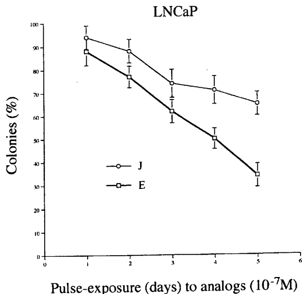
Figure 3. Pulse-exposure of LNCaP prostate cancer cells to analog E. LNCaP cells were exposed for various durations to analog E (10 -7 M). The cells were then thoroughly washed twice, plated into soft agar, and colonies were counted 14 days after plating. Results are the mean of 3 independent experiments and are expressed as a mean percentage \pm SD of control plates that received the same treatment but were not exposed to analog.
