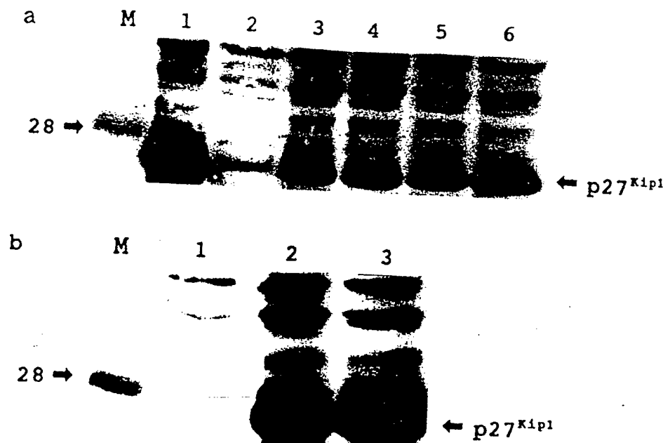
Fig. 5. Western blot analysis of p27 Kip1 levels in MCF-7 and SK-BR-3 cell lines. a : Lane M, marker (in thousands); Lane 1, MCF-7 cells exposed to LH (10 -7 M, 6 days); Lane 2, untreated HL-60 cells. Lane 3, untreated SK-BR-3 cells. Lanes 4, 5, and 6, SK-BR-3 cells exposed to LH (10 -7 M) for 1, 2, and 3 days, respectively. b : Lane M, marker (in thousands); Lane 1, untreated HL-60 cells; Lane 2, untreated MCF-7; Lane 3, MCF-7 cells exposed to LH (10 -7 M, 6 days). Whole-cell extracts were prepared, and equal amounts of protein were loaded into each lane. Blots were then probed using the monoclonal antibody p27 Kip1 and visualized using the ECL system.
