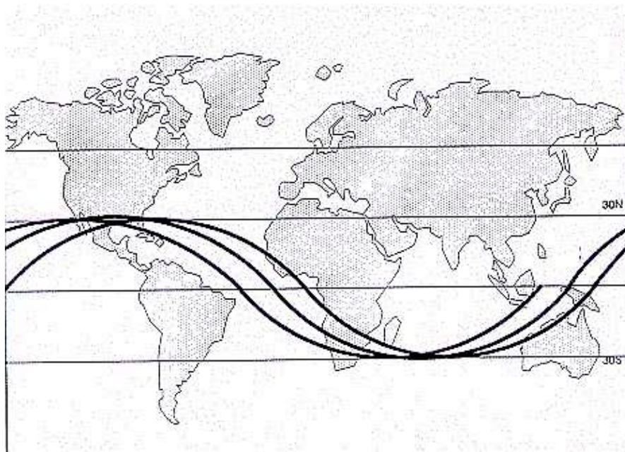
Figure 3. Figure: Satellite Ground Tracks
