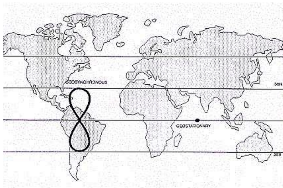
Figure 2. Geosynchronous Ground Tracks
