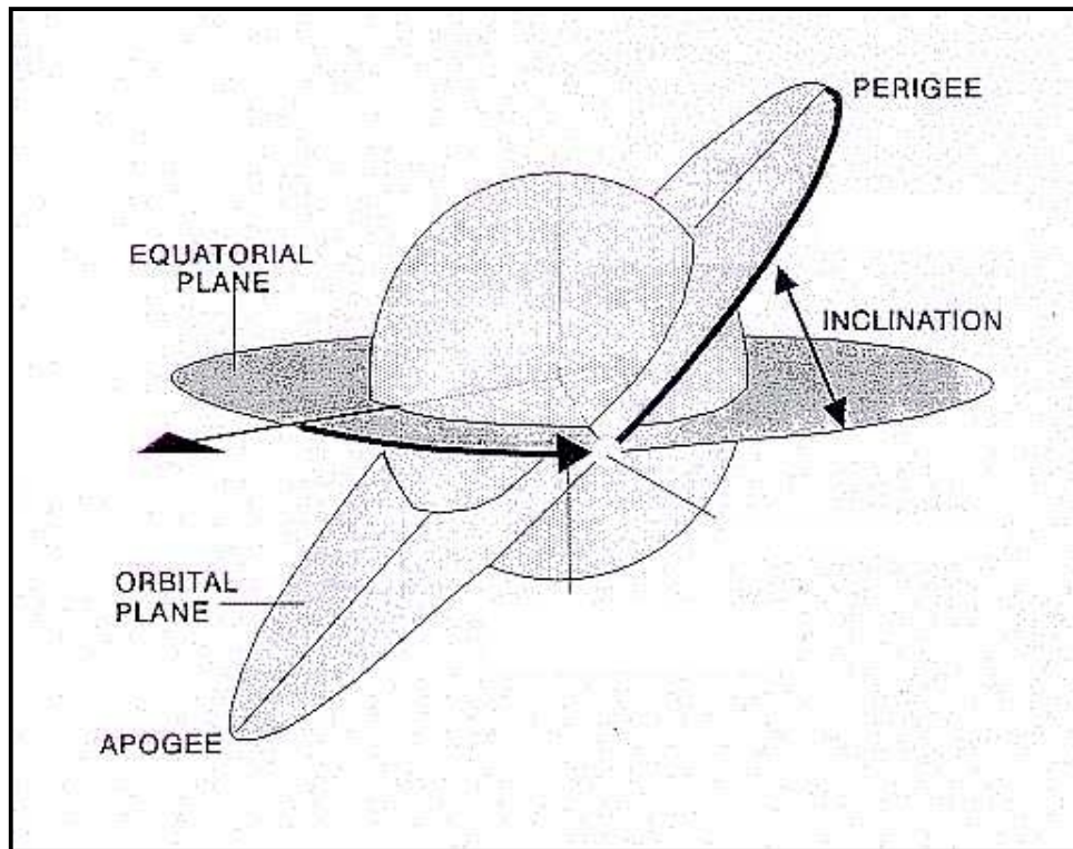
Figure 1: Orbital Terms
