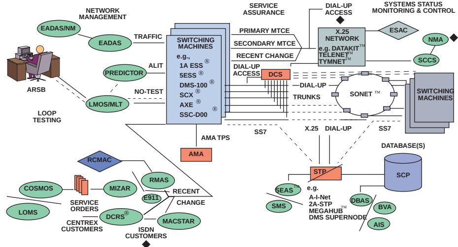
Figure 1. Typical Network Implementation and High Speed Entry Points (◆)
