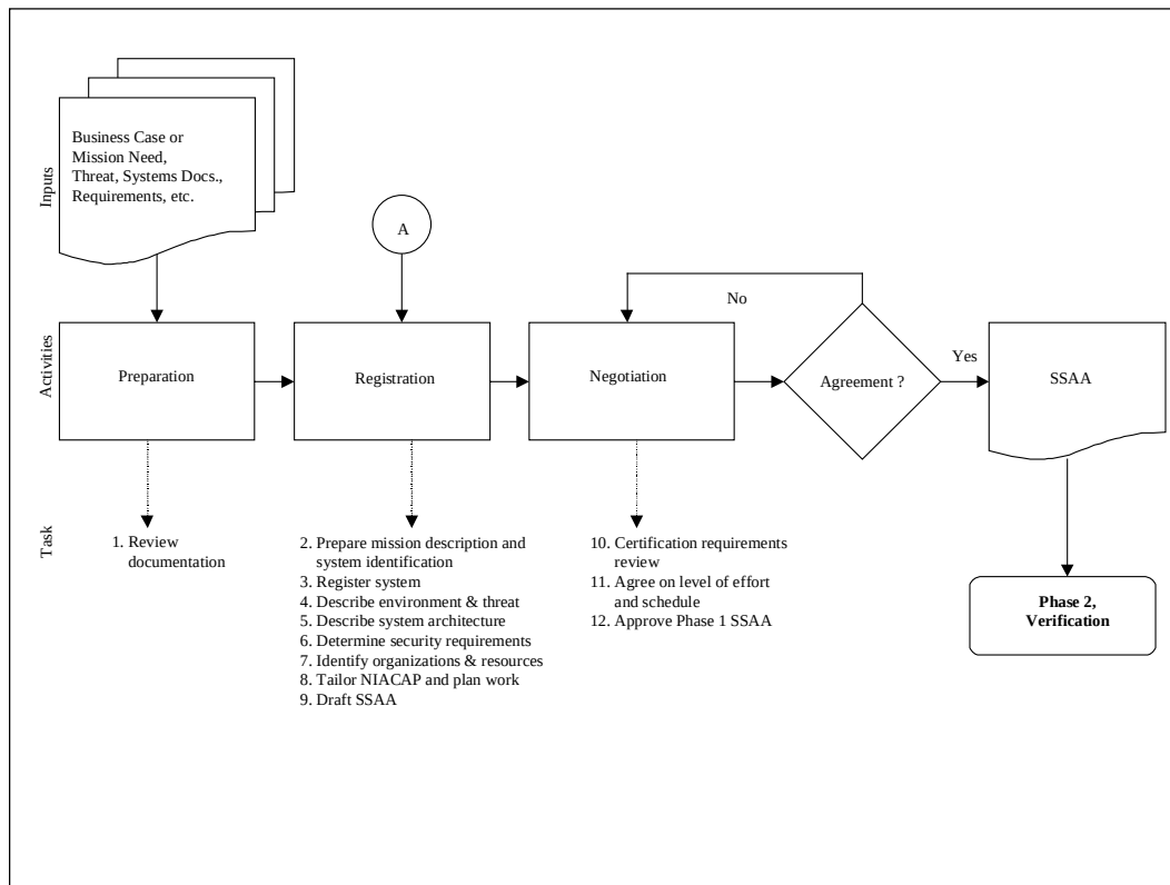
Figure 2. NIACAP Phase 1, Definition
