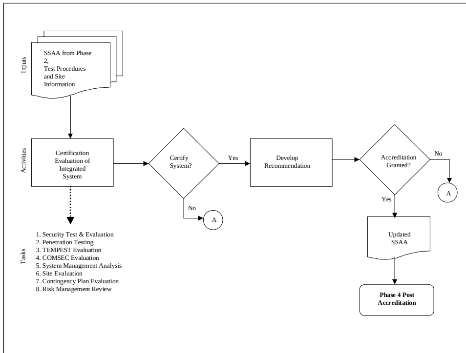
Figure 4. NIACAP Phase 3, Validation
