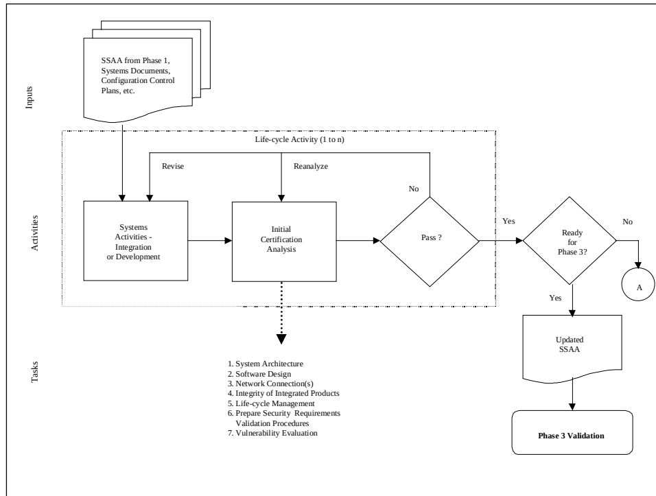
Figure 3. NIACAP Phase 2, Verification
