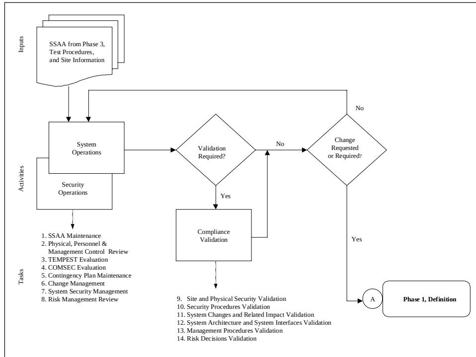
Figure 5. NIACAP Phase 4, Post Accreditation
