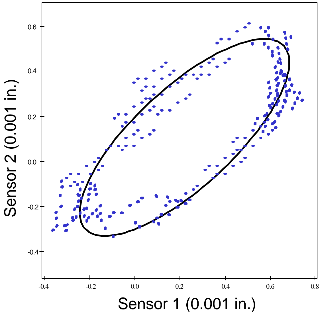
FIGURE 53. Heath's Method Applied to Determine Blade Resonance: Least Squares Fit to an Ellipse
