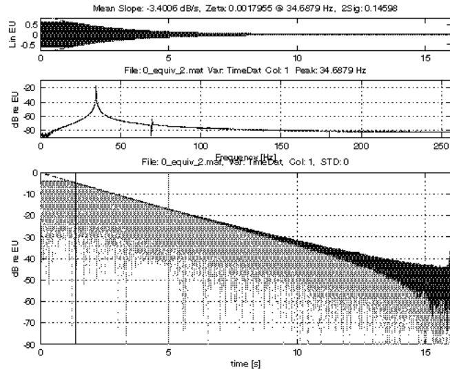
FIGURE 81. Hilbert Transform for Beam with Zero Particles
