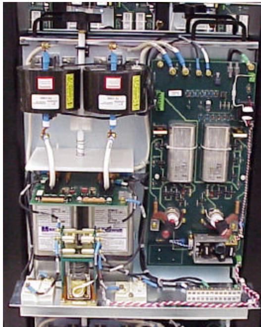
FIGURE 9. One of 48 PFNs That Are Being Integrated into the Laser System
