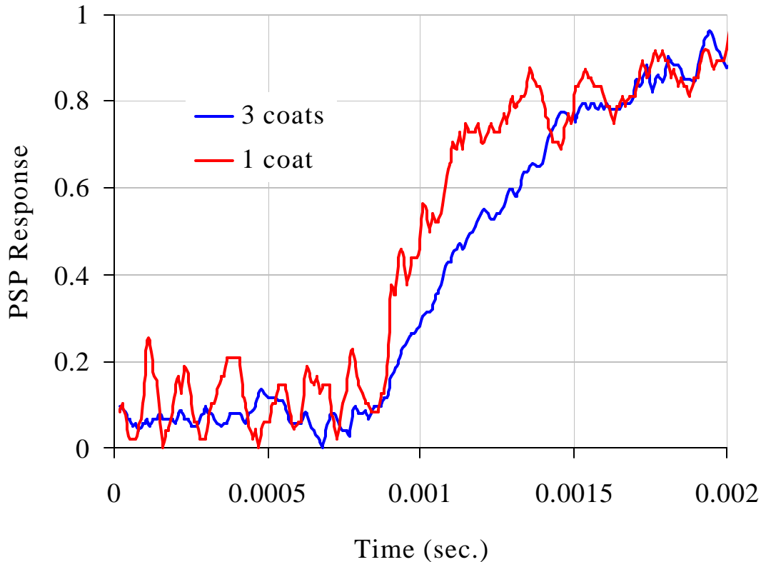
FIGURE 55. Response of Sol-Gel on DuPont to the Initial Shock Wave in the Shock Tube
