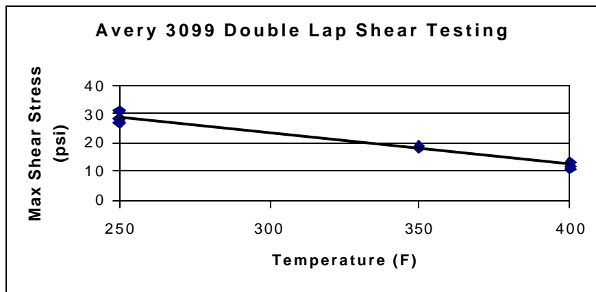
FIGURE 92. Shear Stress
