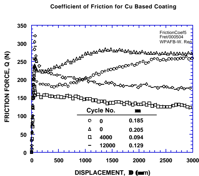
FIGURE 19. Cyclic Evolution of Friction Force for Copper-Based Coating System
