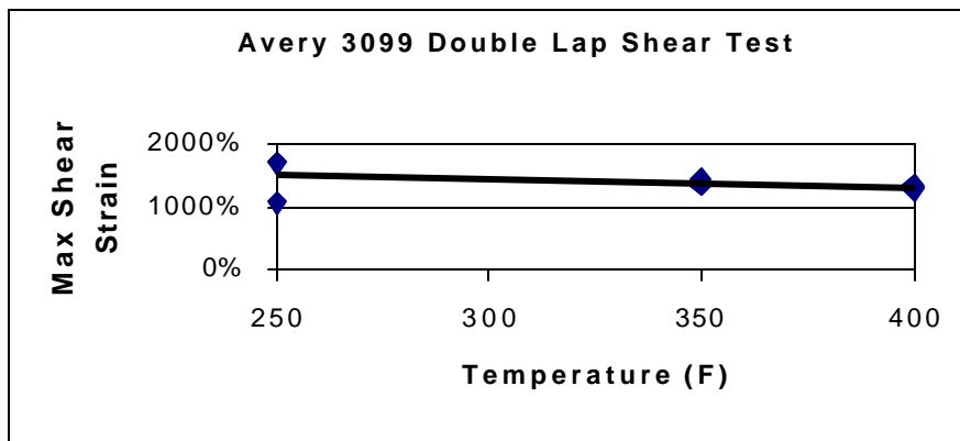
FIGURE 93. Shear Strain
