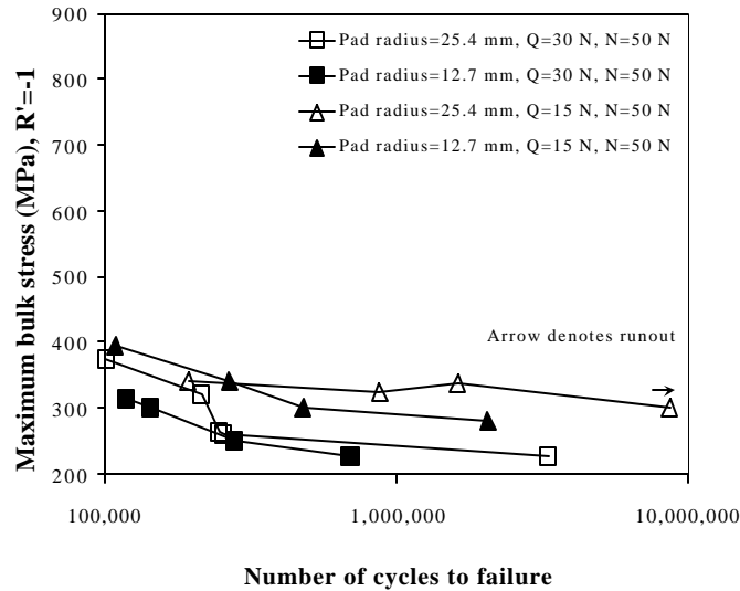
FIGURE 33. Fretting Fatigue Results from Experiments on Mill Annealed Ti-6Al-4V Illustrating Variation of Total Life with Changes in the Bulk Stress Applied to the Specimen
