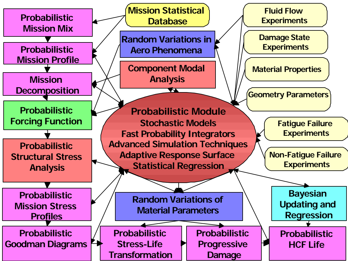
FIGURE 63. Probabilistic HCF Prediction Flowchart
