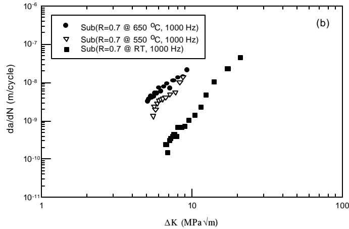
FIGURE 28. Fatigue-Crack Propagation Curves for Fine-Grained KM4 at 25°, 550° and 650°C
