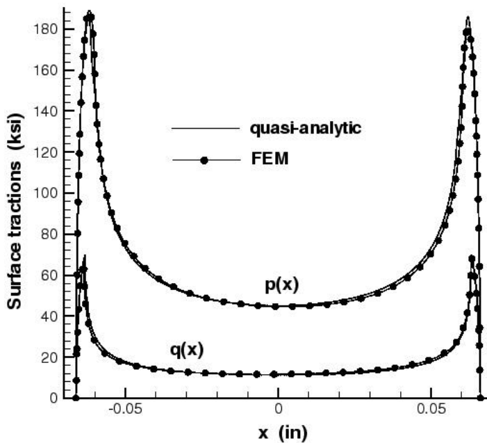
FIGURE 40. Comparison of Surface Normal Tractions Obtained from Integral Equation and FEM Methods
