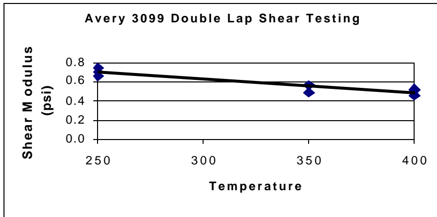
FIGURE 91. Shear Modulus
