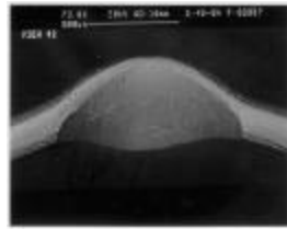
FIGURE 37. Representative FOD from Ballistic and Solenoid Gun Impacts (Sharp Leading Edge Specimens, 30° Impacts, High Damage Levels)
