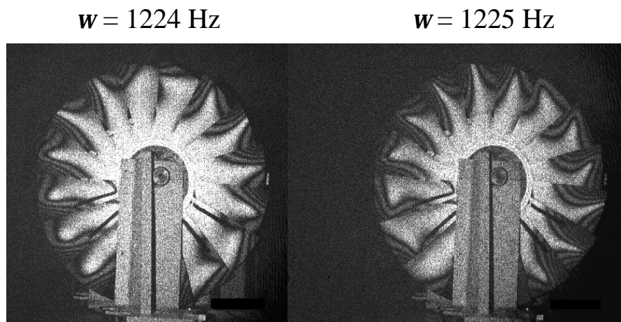
FIGURE 103. 2B/1T Mode Interaction.
