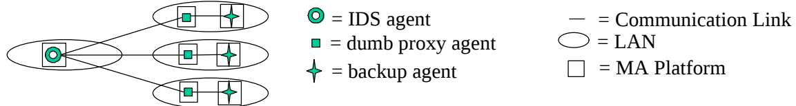
Figure 3: The Communication and Location Model for Agent Backups
