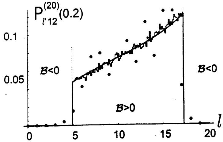
Figure 1: The Monte-Carlo simulation (step-like lines), the classical (solid line) and quantal (dots) transition probabilities P_{\ell'\ell}(\alpha) for a given Stark parameter \alpha = 0.2 and initial \ell = 12 within the n = 20 shell. \mathcal{A} < 0 for all \ell' .
