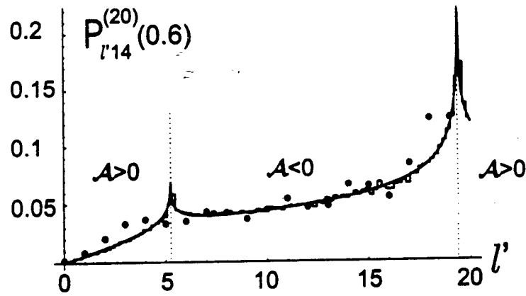
Figure 2: The Monte-Carlo simulation (step-like lines), the classical (solid line) and quantal (dots) transition probabilities P_{\ell'\ell}(\alpha) for a given Stark parameter \alpha = 0.6 and initial \ell = 14 within the n = 20 shell. \mathcal{B} > 0 for all \ell' .
