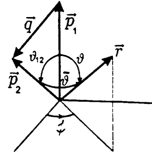
FIG. 13. The basic geometry for calculation of \mathcal{R}_{if} .
