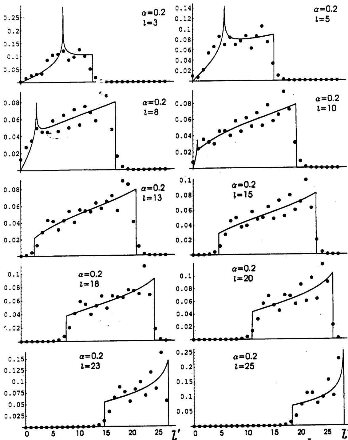
FIG. 14. The classical and quantal Stark mixing transition probabilities P_{\ell' \ell}(\alpha) within the n=28 energy shell, for \alpha=0.2 , as a function of the final angular momentum \ell' and for various initial angular momenta \ell .
