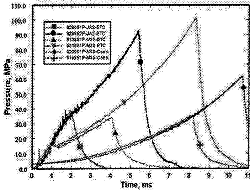
Figure 7. P-t Curves for Plasma-Ignited M30 (Mylar Capillary) and JA2 (PE Capillary) Firings, Along With Conventional Firings for M30, for Interrupted Closed-Bomb Trials.
