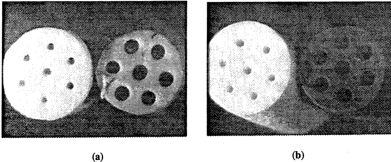
Figure 8. Samples: (a) Conventionally Ignited With Black Powder and (b) Plasma-Ignited With Mylar-Based Capillaries.
