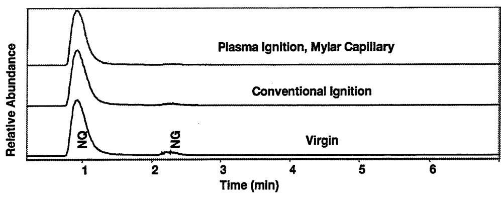
Figure 12. LC-MS Analysis of M30 Samples.
