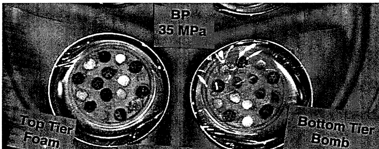
Figure 10. Grains Originally From the Top Tier, Extinguished at 35 MPa; Grains Recovered From the Closed Bomb (Right Side) Are Yellowed, While Grains Recovered in the Foam (Left Side) Are Not Discolored, Except for Modest Residue.
