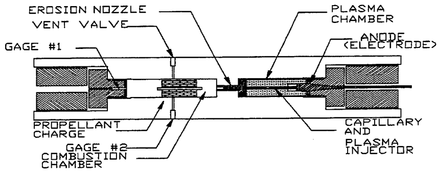
Figure 2. Schematic of the Plasma Igniter.
