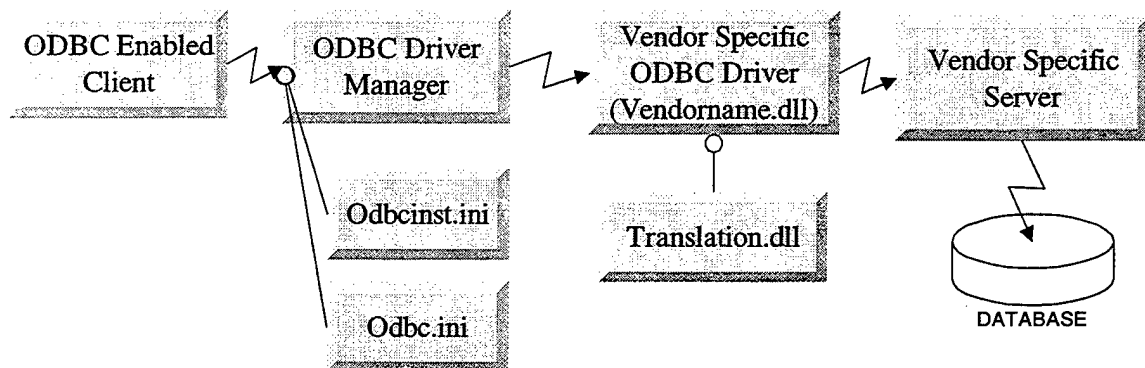
Figure 4.3 ODBC Architecture
