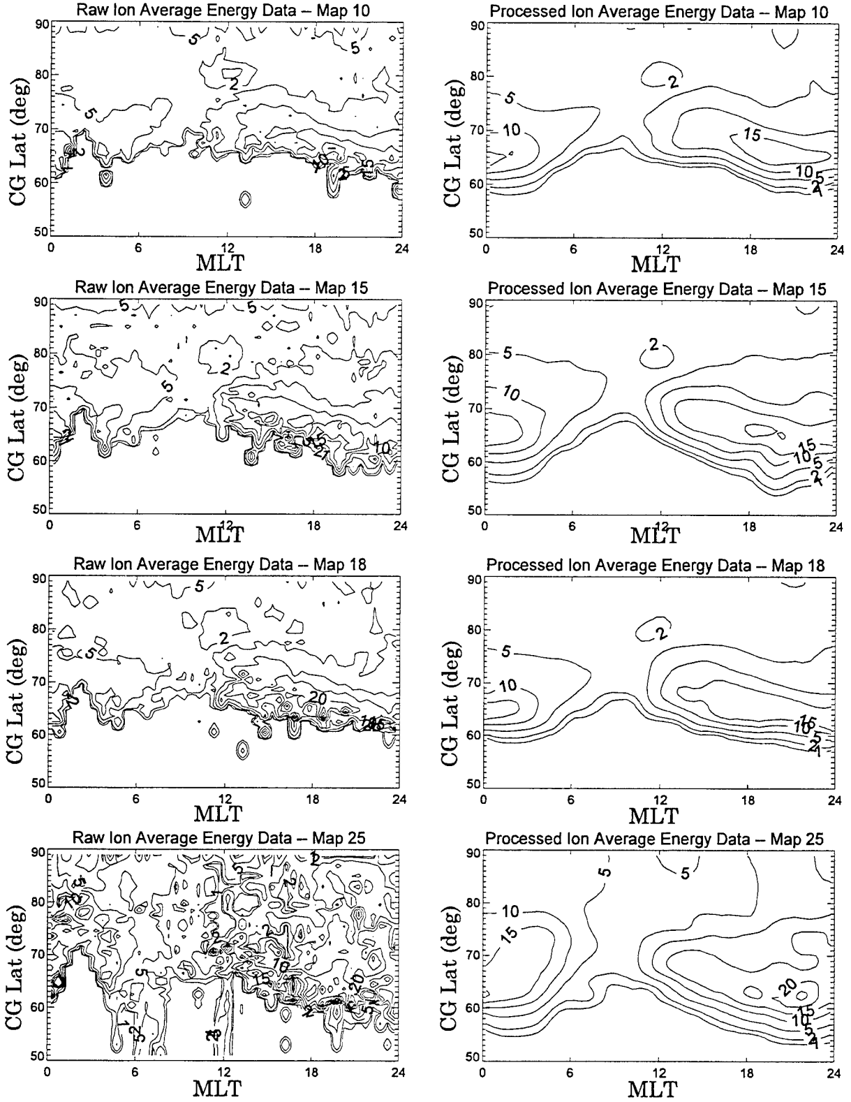
Figure 10. Same as Figure 9 Except for the IMF/SWS Ion Average Energy (in keV).
