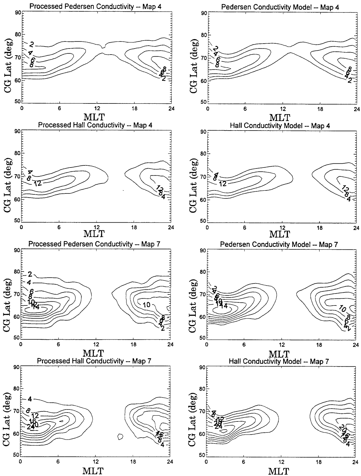
Figure 34. Comparisons Between Smoothed Data and Model for the Conductivities from the K_p Maps (in mhos).
