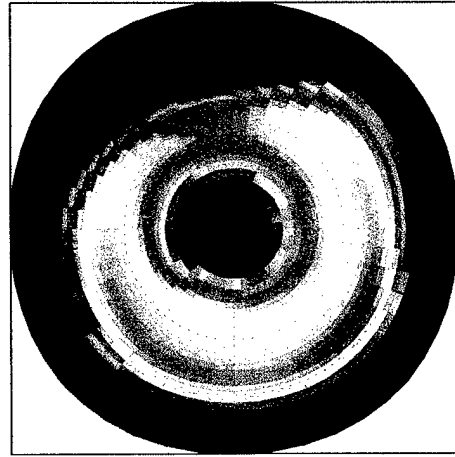
New Electron N-flux for Kp
