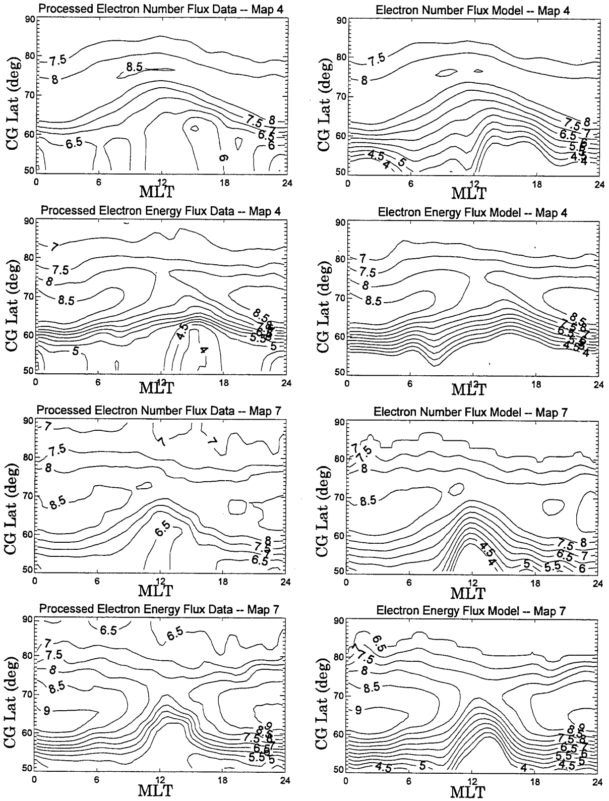
Figure 29. Same as Figure 28 Except for the K p Electron Number and Energy Flux.
