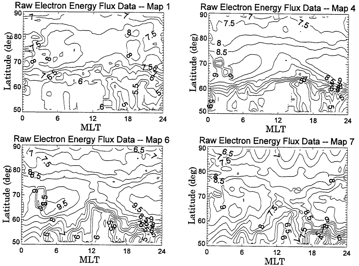
Figure 2. Contours of \log_{10} Raw Electron Energy Flux (In \text{keV-cm}^{-2}\text{-sr}^{-1} ) for the Most Populated K_p Map and the Three Least Populated Ones, According to Total Number of Samples in the K_p Division.
