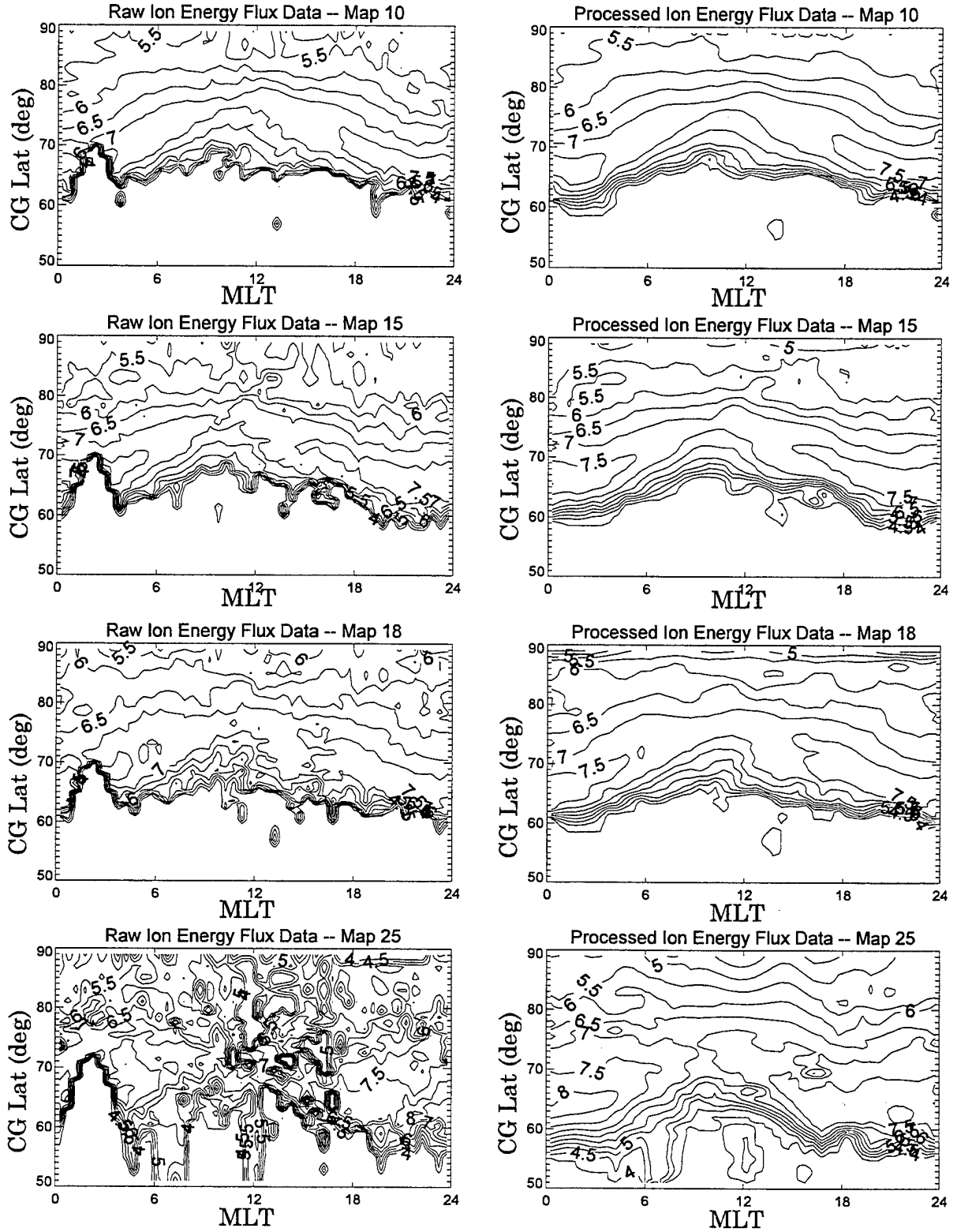
Figure 9. Same as Figure 8 Except for the Ion Energy Flux (in \text{keV/cm}^2\text{-s-Sr} ).
