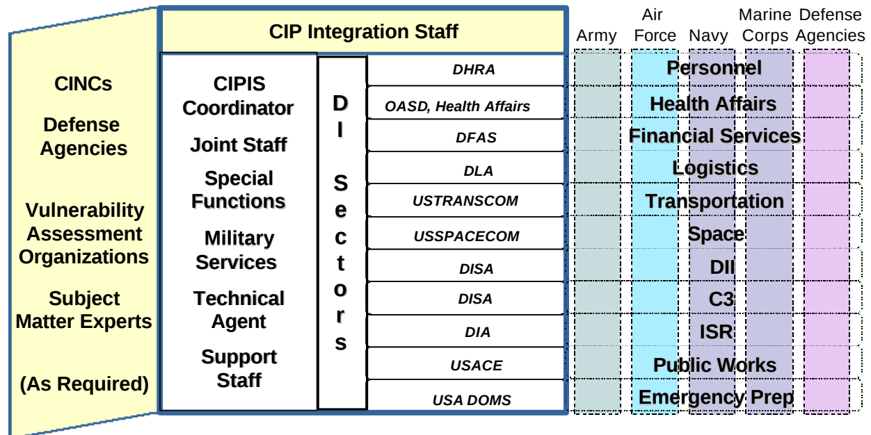
Figure 2 – CIPIS Structure
