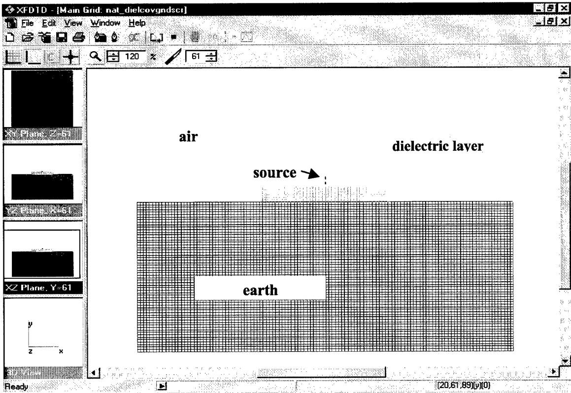
Figure 3-1(b) XFDTD model of dielectric layer covered ground screen
