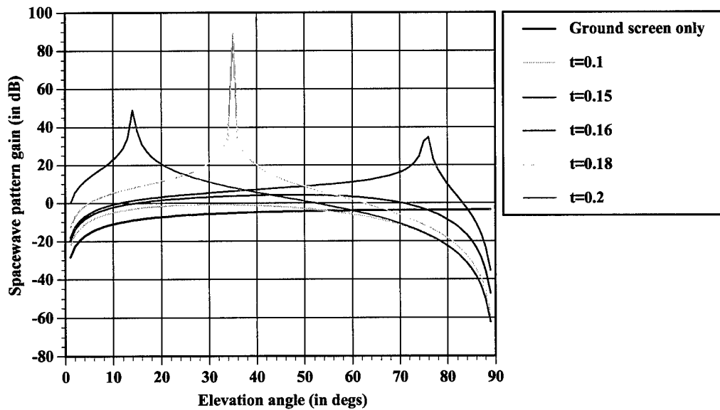
Figure 4.3-8 Computed elevation patterns with dielectric layer on ground screen computed as a function of dielectric thickness
