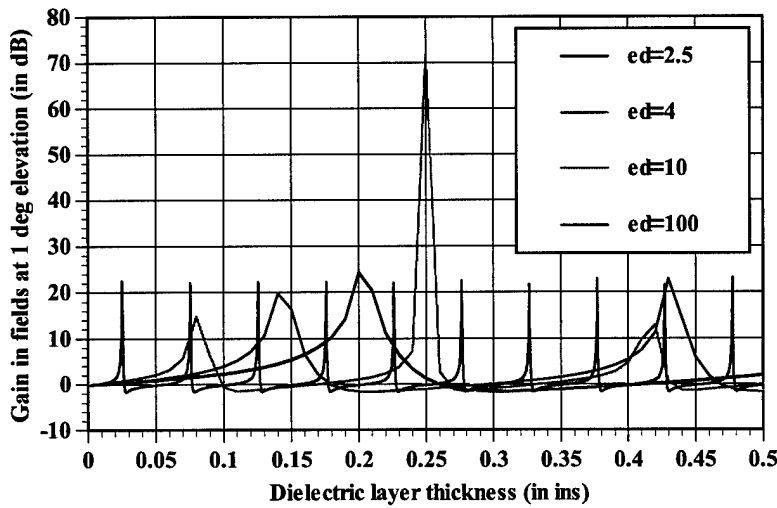
Figure 4.3-5 Computed gain enhancement with dielectric layer compared to ground screen only as a function of layer dielectric constant Screen diameter = 4", \epsilon_1=4.0 , \sigma_1=0.0
