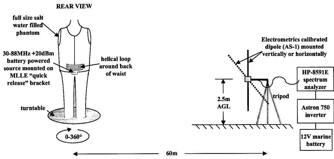
Figure 6-1 Recommended setup for measuring power gain
