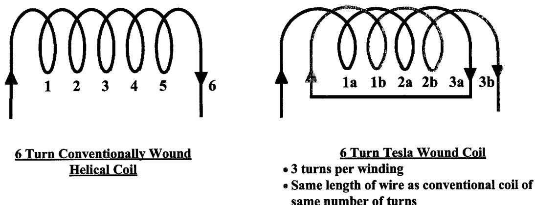
Figure 4.2-5 Comparison of winding configurations for conventionally and Tesla wound coils of the same number of turns
