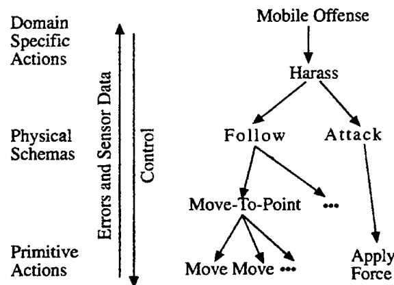
Figure 5. HAC action form a hierarchy, control information is passed down, messages and sensor integration occurs bottom-up
