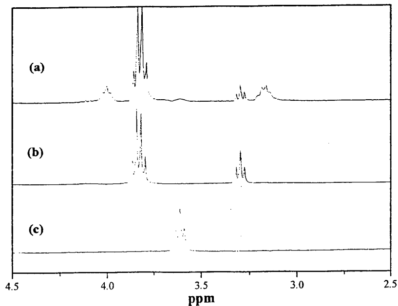
Figure 15-II. ^1\text{H} NMR of urethane-forming reaction: (a) crude product after 12 h reaction time (25 °C), (b) \gamma -isocyanatopropyl triethoxysilane, (c) alcohol-terminated PIB precursor.
