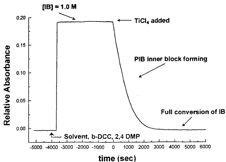
Figure 4-II. Profile of isobutylene monomer depletion over time, from analysis of absorbance at 887 \text{ cm}^{-1}
