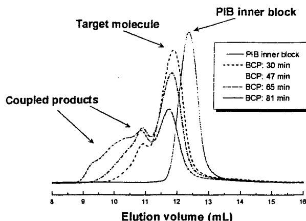
Figure 9-II. GPC traces (refractive index detector) of aliquots taken at various times during styrene polymerization.
