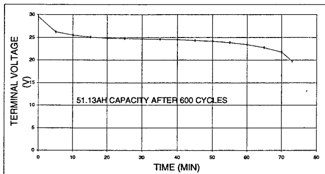
Figure 11. CAPACITY CHECK AFTER 600 CYCLES, 42 Ah SEALED LIFE TEST BATTERY, 42 AMPERE DISCHARGE @ 21 DEG. C
