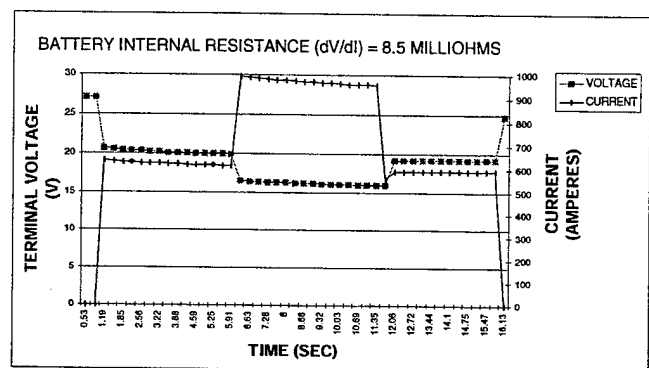
Figure 18. 42 Ah SEALED LIFE TEST BATTERY INTERNAL RESISTANCE CHECK @ 21 DEG. C AFTER 1000 CYCLES
