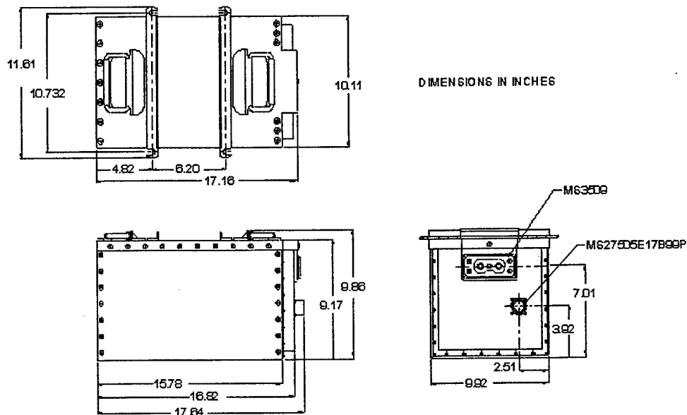
Figure 2-3. Battery Outline Dimensions & Interfaces
