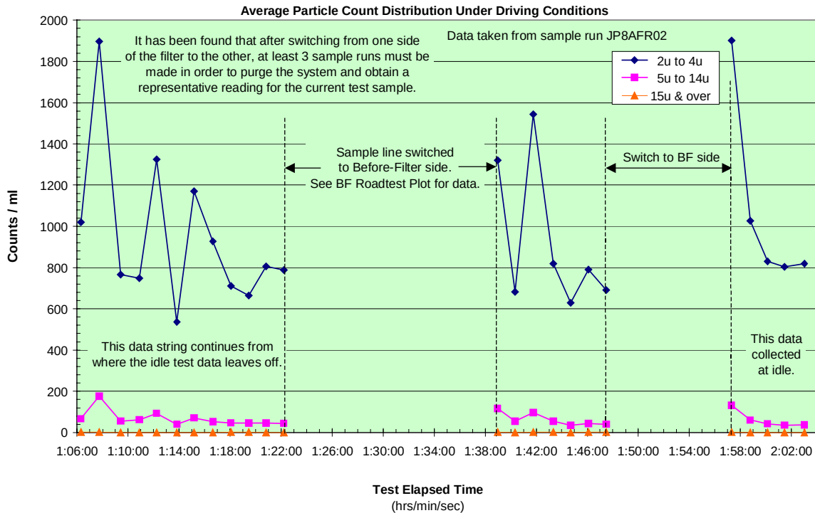
Figure 8. CS500 HMMWV JP-8+100 After-Filter Road Test Data
