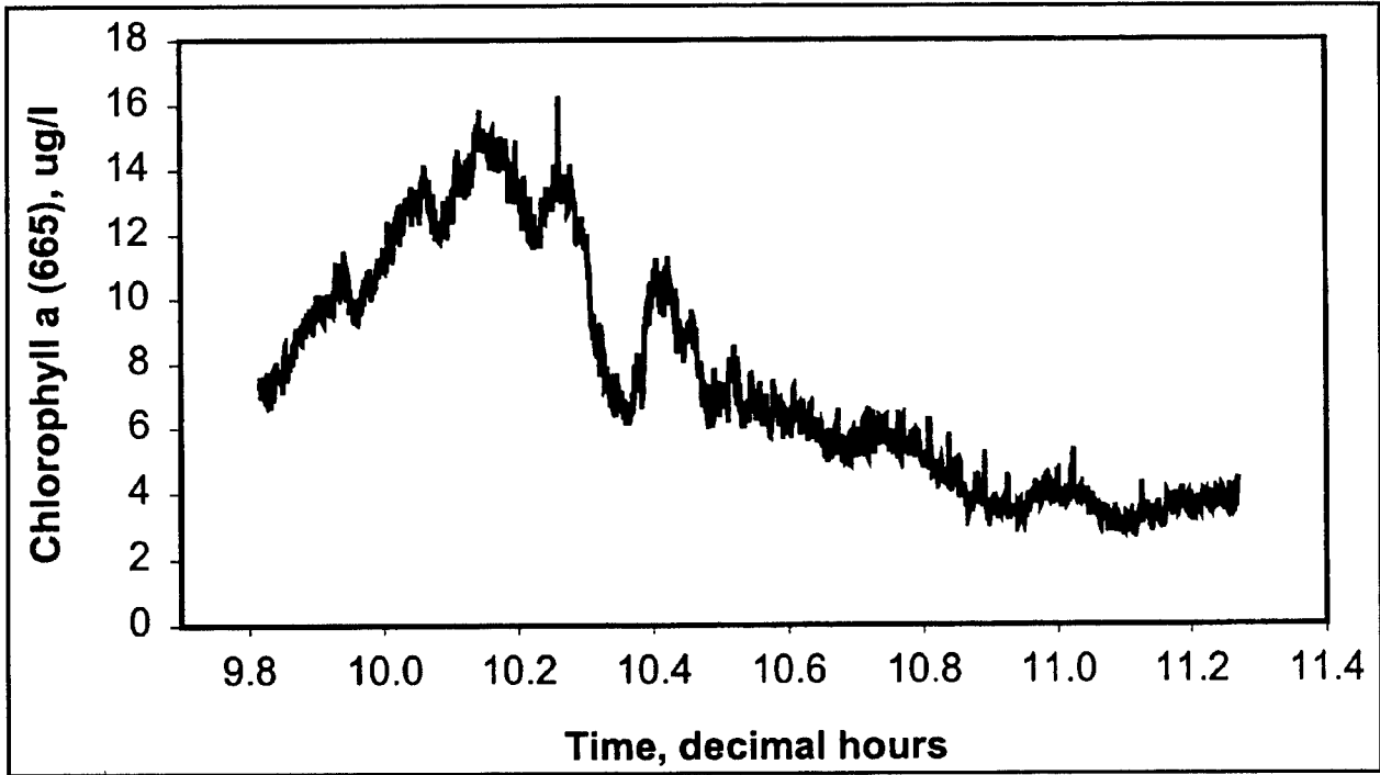
Figure 4. Variation of chlorophyll a throughout an extensive reach of the Kanawha River. In this plot, travel velocity was relatively constant and time may be loosely interpreted in terms of distance. The substantial variation observed in this study may not have been discovered using conventional methods. Using this approach, the only limitation to the distance traveled during one day was the speed of the watercraft and the data interval required by study goals
