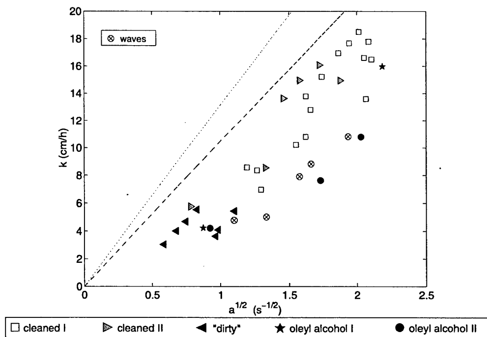
Figure 7-32: Dependence of the gas-transfer velocity on surface divergence for grid-stirred turbulence and mechanically generated surface waves. The Lewell and Csanady curves are as before. The uncertainty for the grid turbulence data is as in figure 7-28; the uncertainty for the waves data ranges from \pm 0.5 \text{ s}^{-1/2} to \pm 0.9 \text{ s}^{-1/2} . R^2 = 0.77 .
