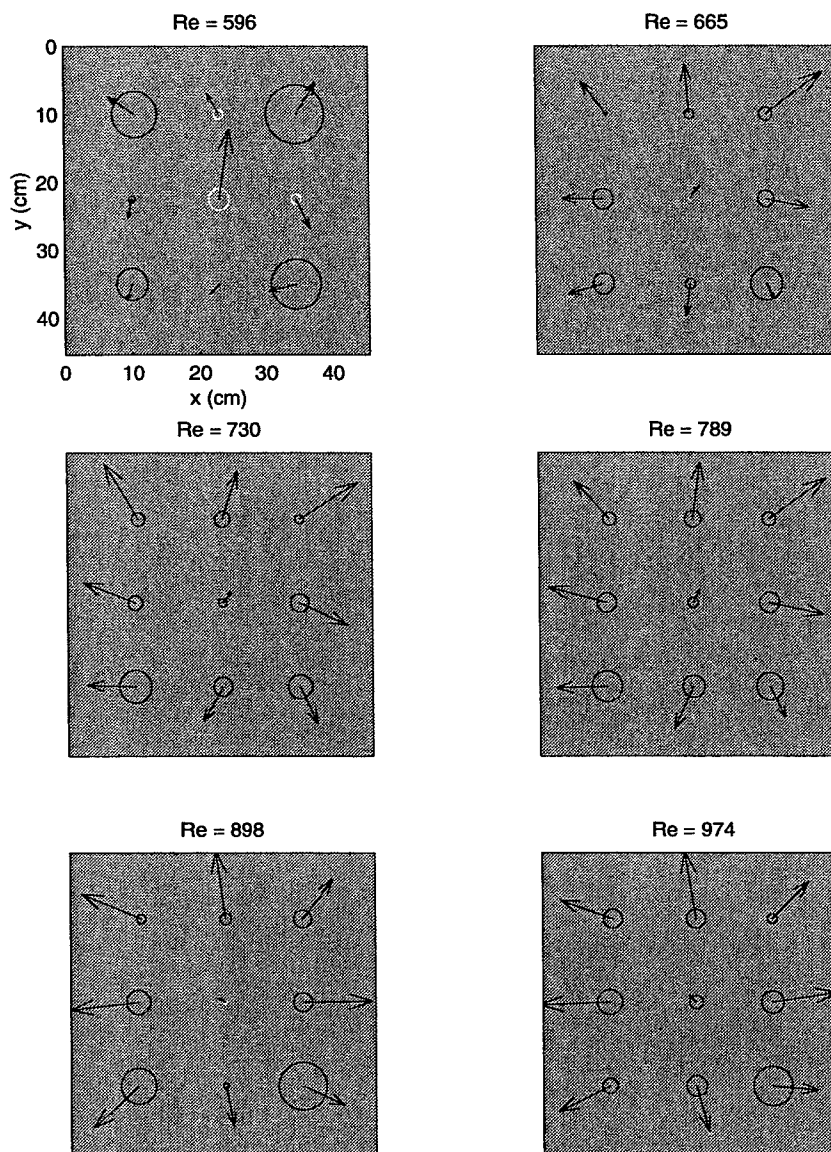
Figure 6-11: Spatial variability of mean flow components measured at a depth of 8 cm for grid A. See figure 6-10 caption for details.
