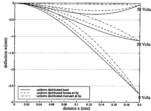
Figure 2 The centreline deflection under various loads
