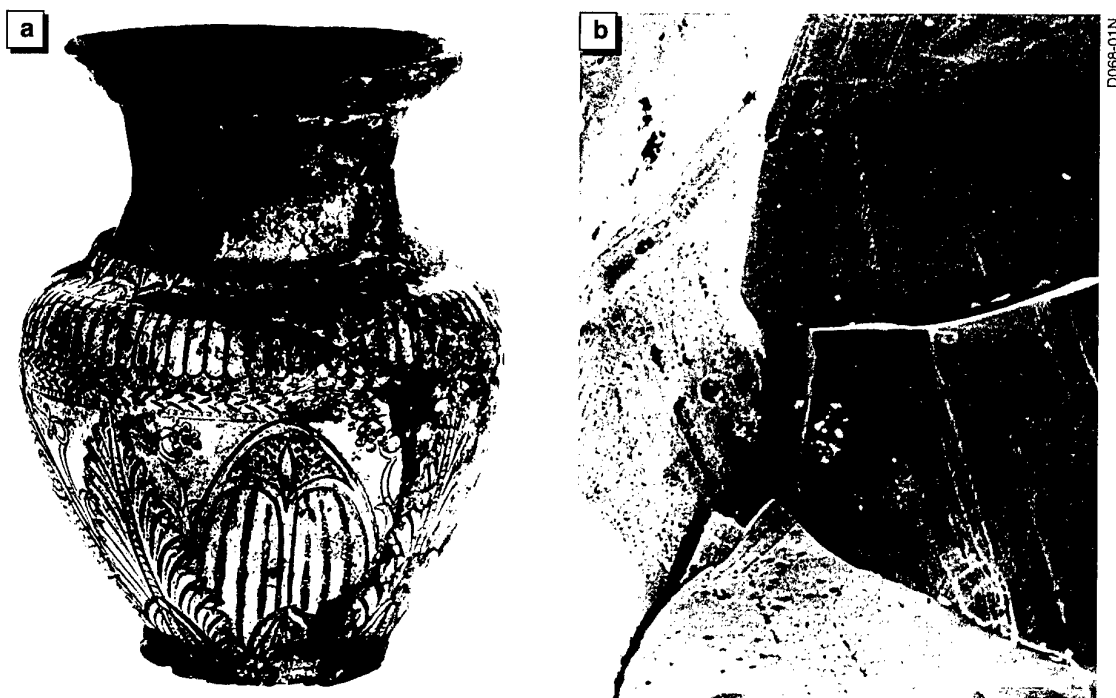
Fig. 3 Brittle grain boundary fracture in a sample from an Egyptian silver vase (Wanhill et al.1998)
