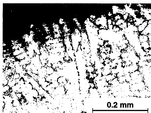
Interdendritic: metallograph (Scott 1996)
