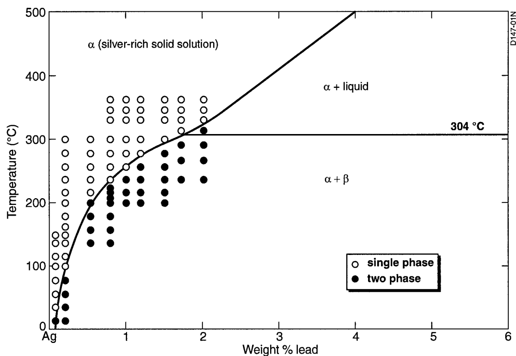
Fig. 1 Silver-rich low temperature region of the Ag-Pb equilibrium phase diagram, determined by ageing supersaturated solid solutions at the indicated temperatures (Thompson and Chatterjee 1954)
