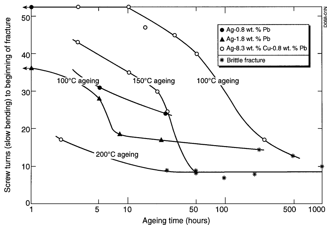
Fig. 2 Age-embrittlement of cast, solution treated and aged Ag-Pb and Ag-Cu-Pb alloys. Data from Thompson and Chatterjee (1954)
