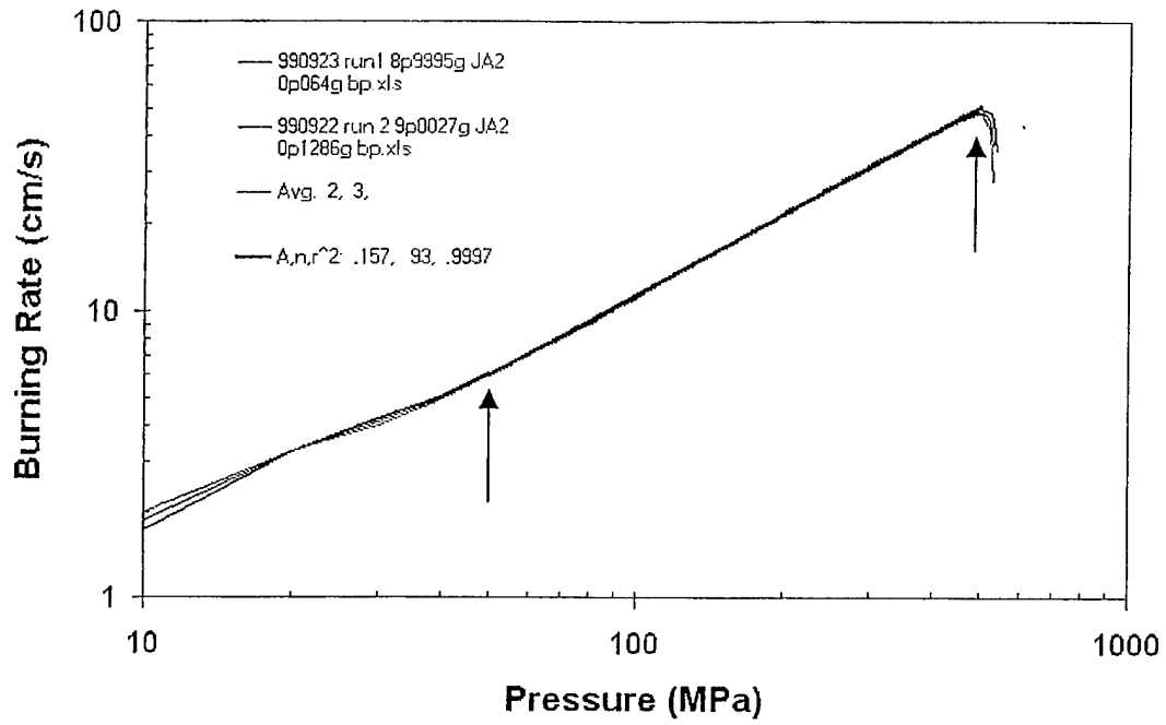
Figure 11. Comparison tool of two JA2 test runs with average and BR law fit.
