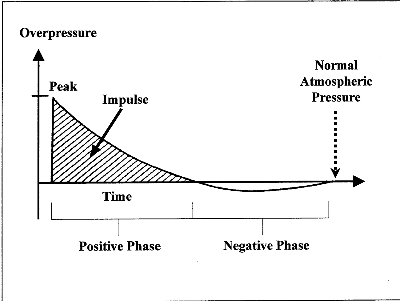
Figure 1: Pressure-Time History of an Air Blast
