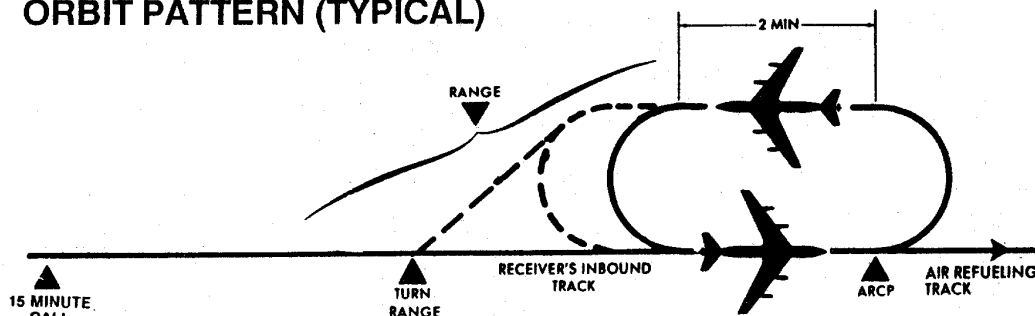
Figure 14: Orbit Pattern (Typical)
