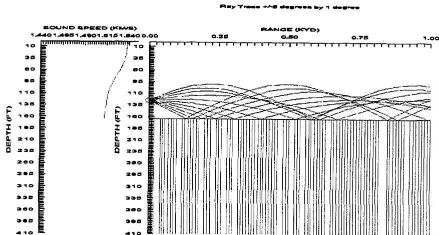
b. Maximum Detection Range (DR) for a Bottom Target Depth = 835 yd, \Delta DR = 225 yd
