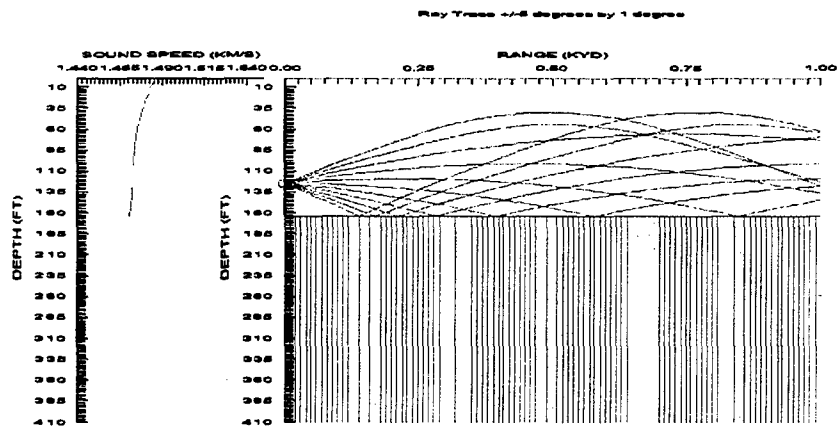
c. Maximum Detection Range (DR) for a 26 ft. Target Depth = 620 yd
