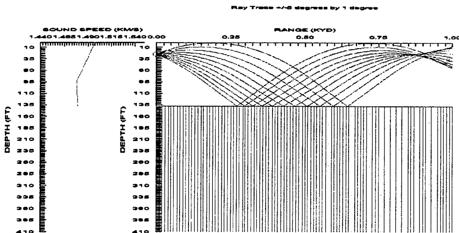
c. Maximum Detection Range (DR) for a 26 ft. Target Depth = 890 yd
