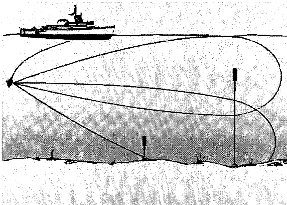
Figure 12. AN/SQQ-32 Concept.
