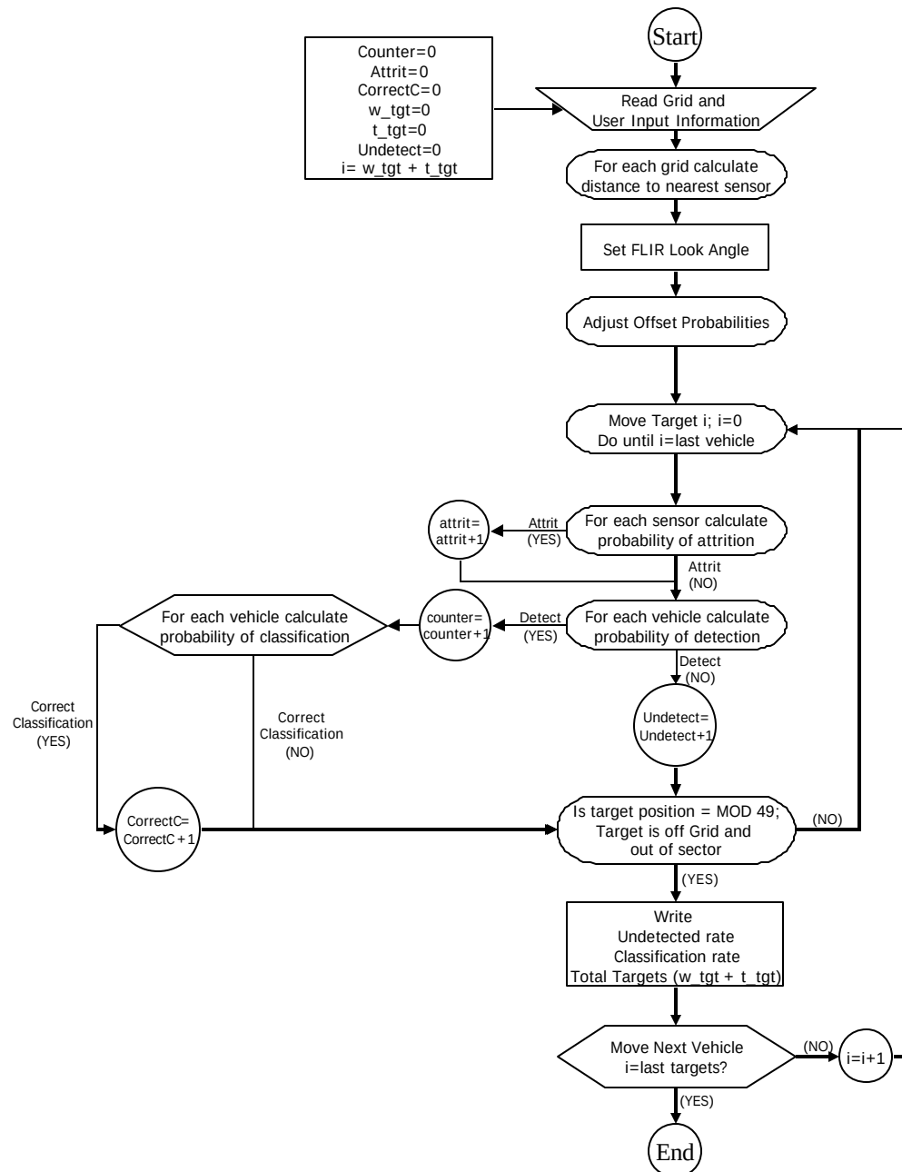
Figure 57: Pseudo Code Schematic
