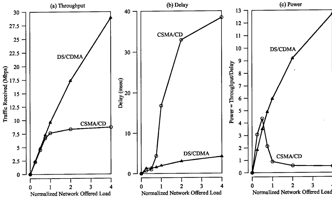
Figure 4.15. Comparison of DS/CDMA and CSMA/CD Responses Vs. Network Offered Load
