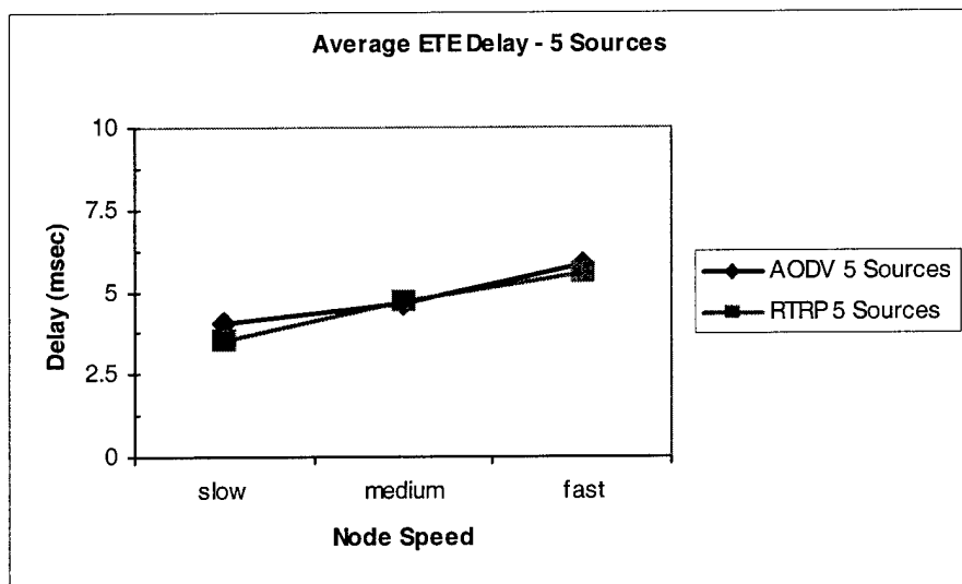
Figure 17. Average ETE Delay for 5 source Nodes
