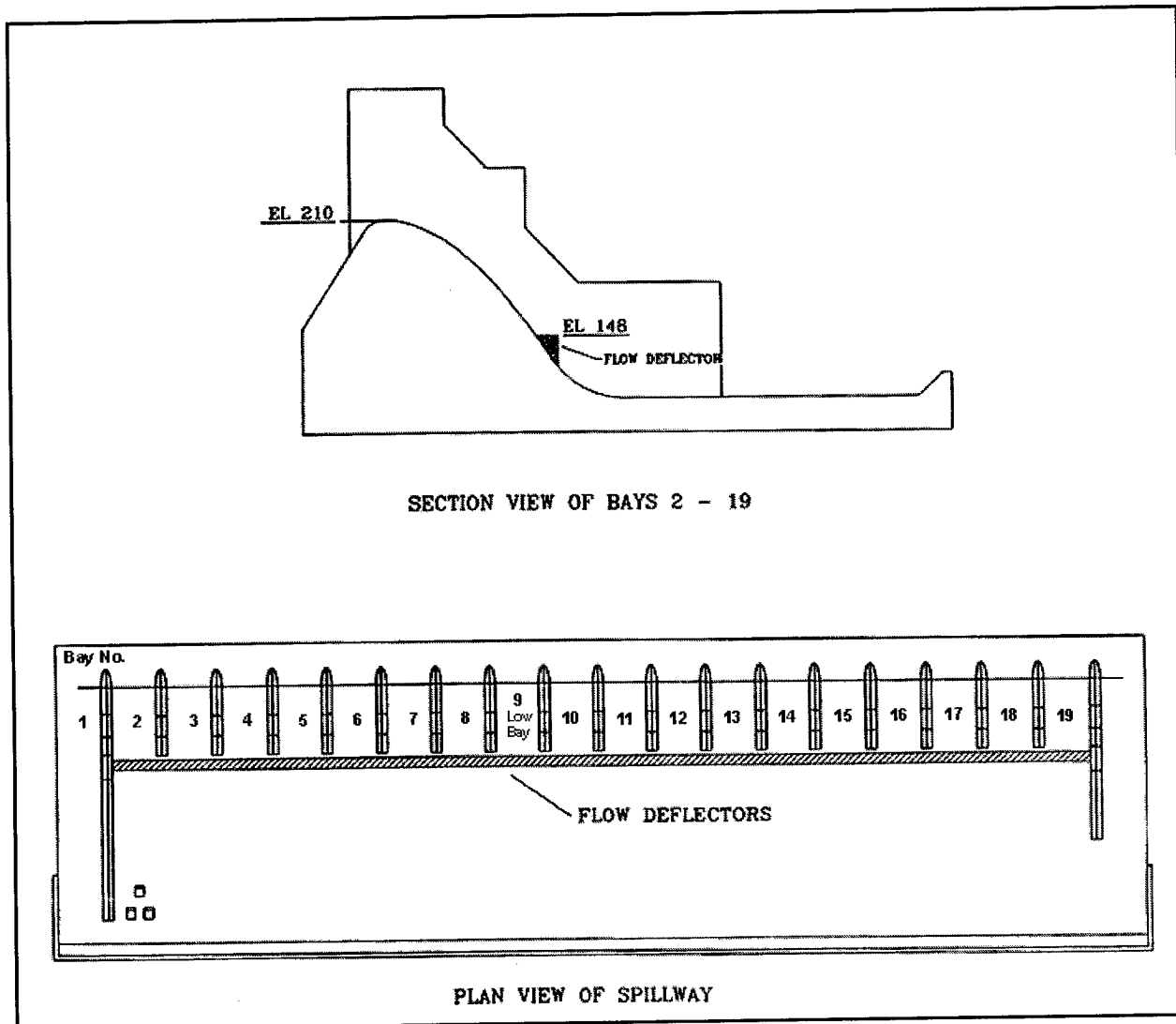
Figure 3. Flow deflector (not to scale)
