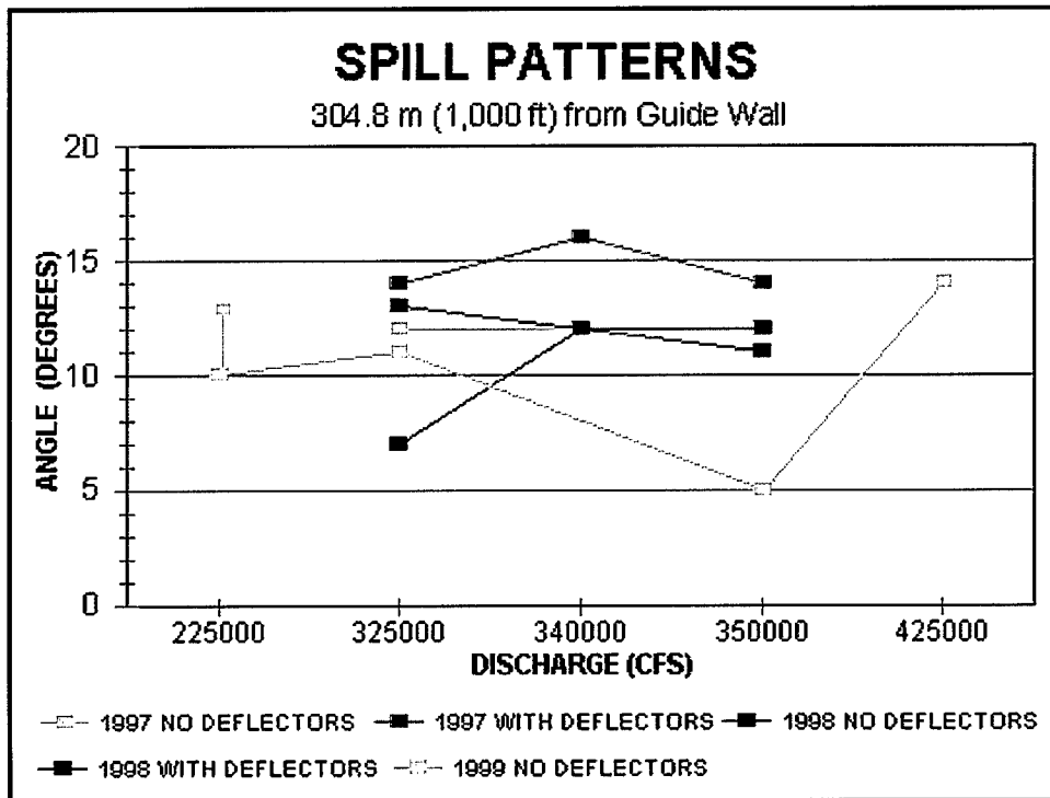
Figure 8. Angle versus discharge plot of flow entering navigation channel 304.8 m (1,000 ft) downstream of guide wall
