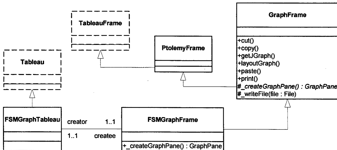
Figure 13.14 Static structure of the Ptolemy graph editor.
