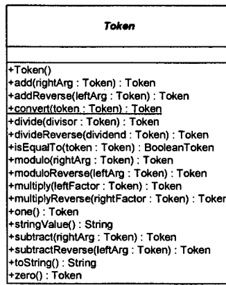
FIGURE 5.3. The Token class defines a polymorphic interface that includes basic arithmetic operations.
