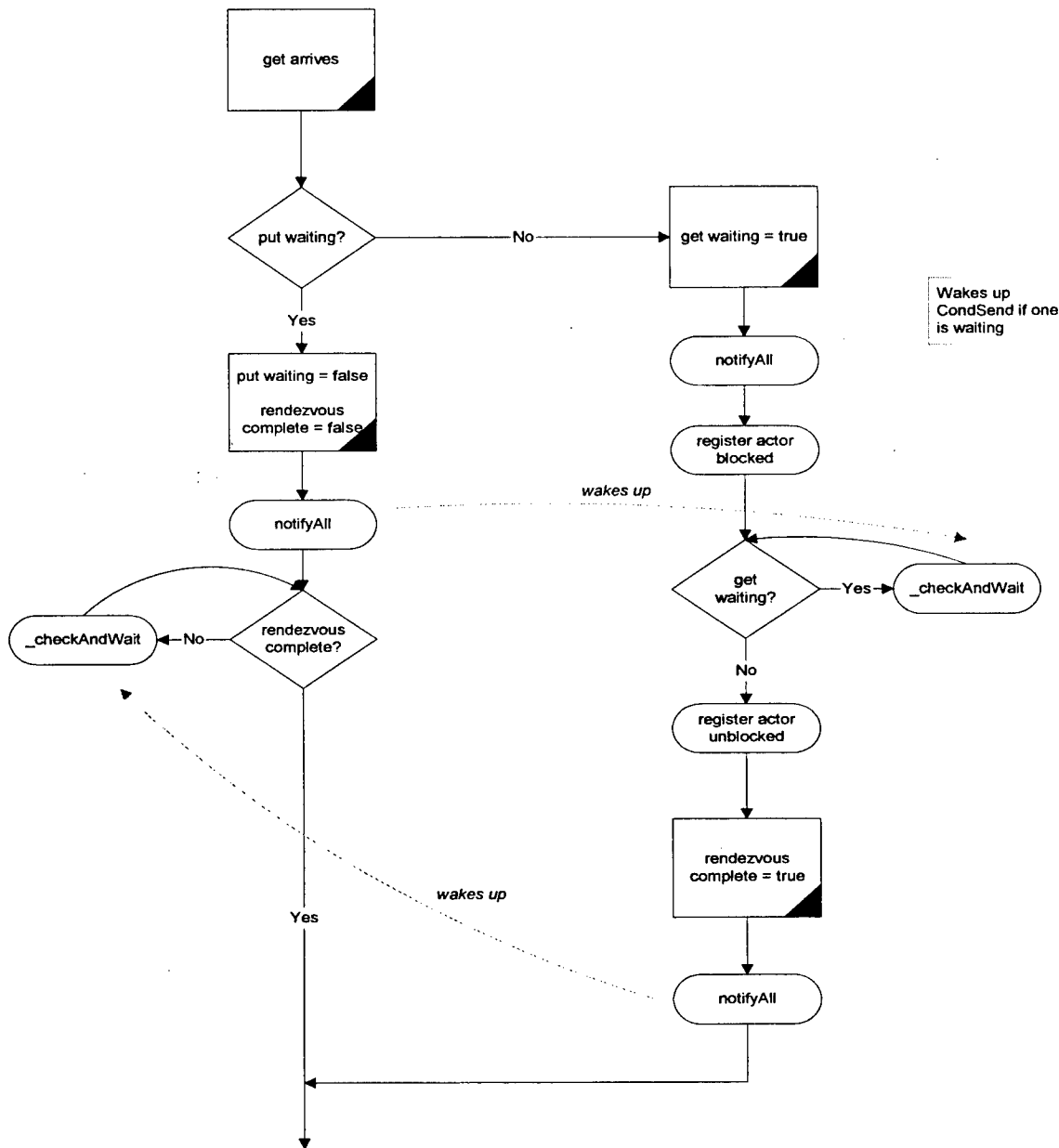
FIGURE 17.12. Rendezvous algorithm.
