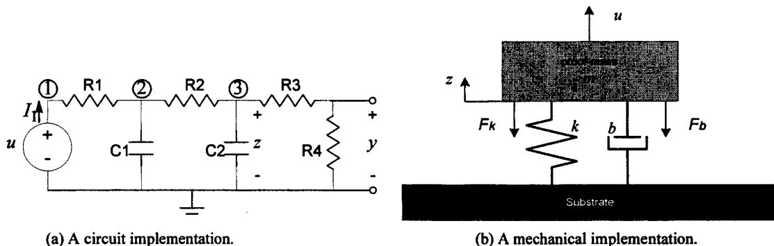
FIGURE 14.1. Possible implementations of the system equations.
