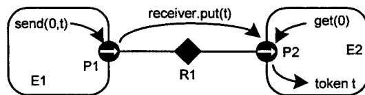
FIGURE 8.1. Message passing is mediated by the IOPort class. Its send() method obtains a reference to a remote receiver, and calls the put() method of the receiver, passing it the token t . The destination actor retrieves the token by calling the get() method of its input port.
