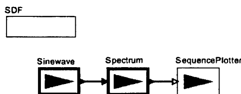
FIGURE 2.12. A multirate SDF model.
