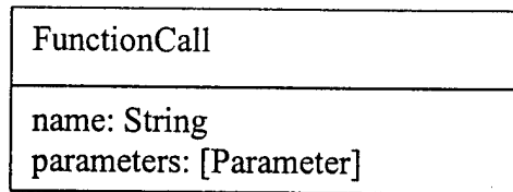
Figure 26 – FunctionCall Type
