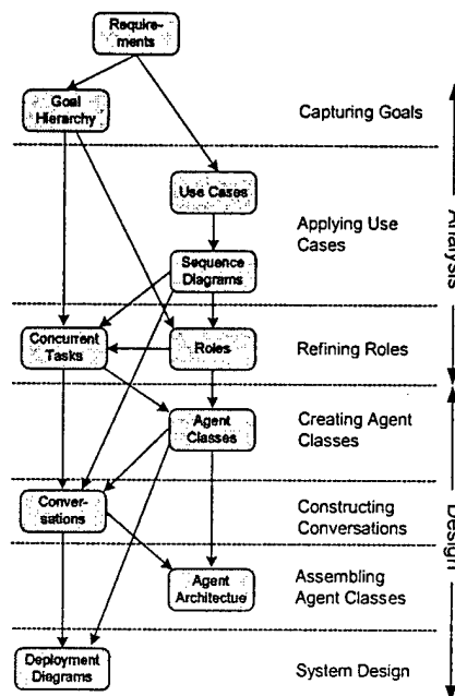
Figure 1 – MaSE Methodology
