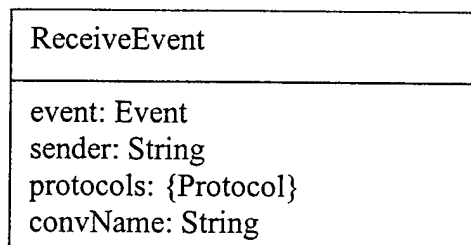
Figure 28 – ReceiveEvent Type
