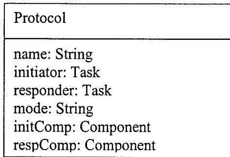
Figure 13 – Protocol Type
