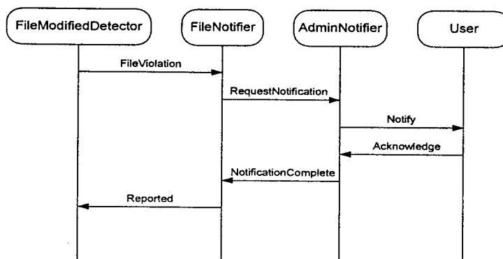
Figure 2 – Sequence Diagram [5]
