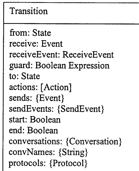
Figure 22 – Transition Type
