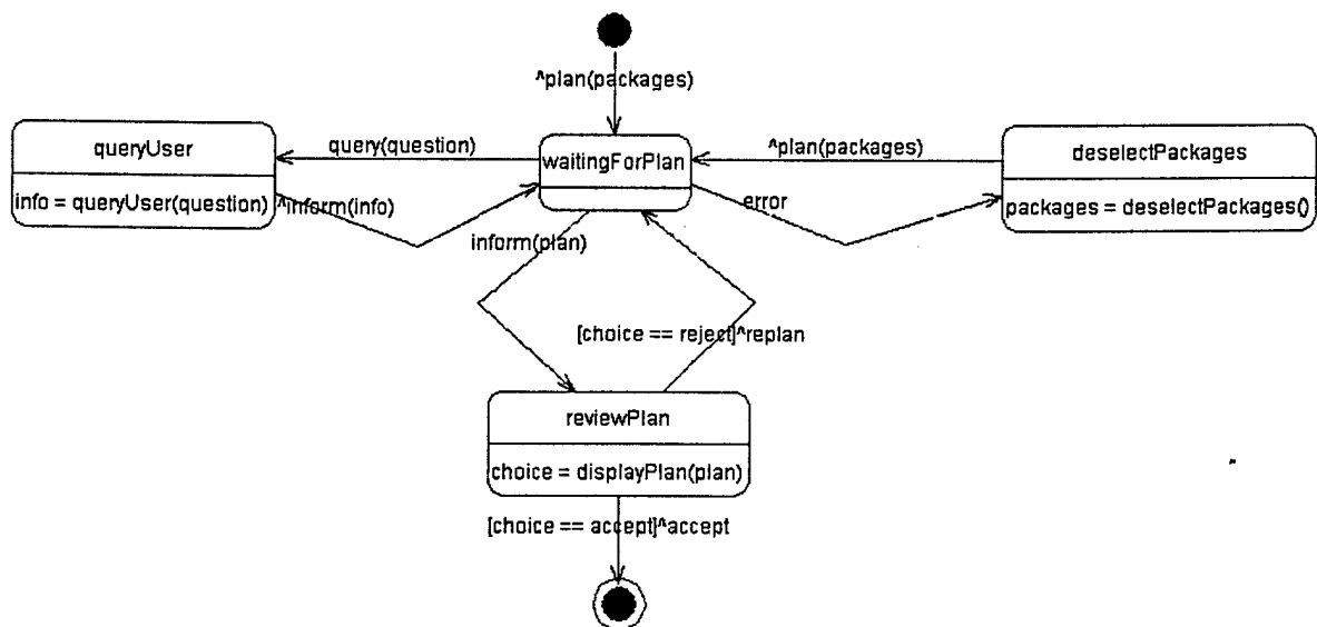
Figure 110 – Communication Class Diagram
