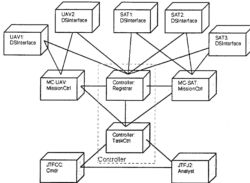
Figure 111 – Deployment Diagram [8]
