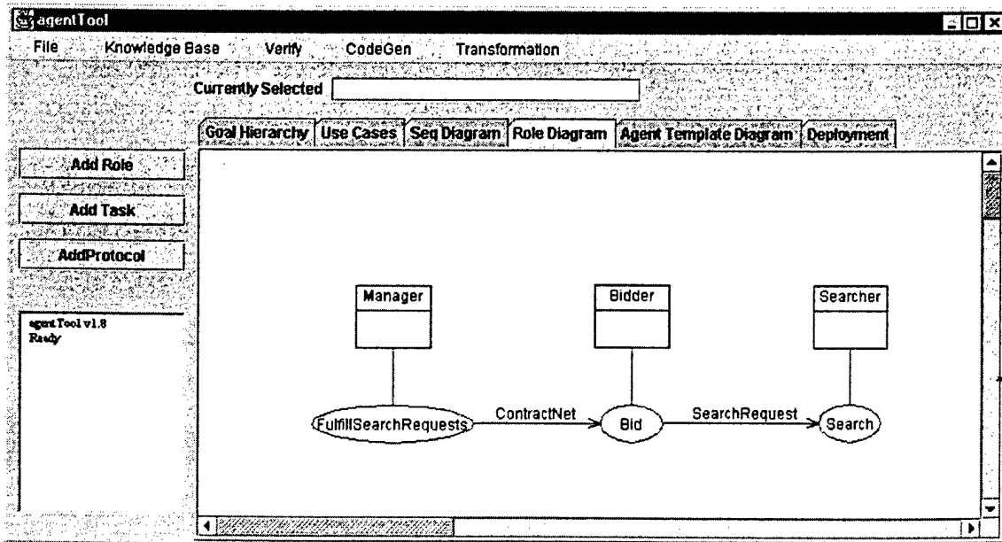
Figure 83 – Role Model
