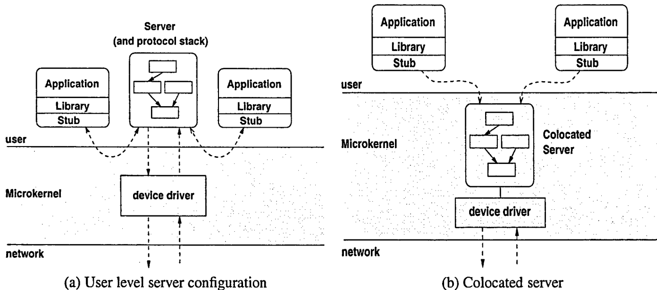
Figure 3: Service implementation.
