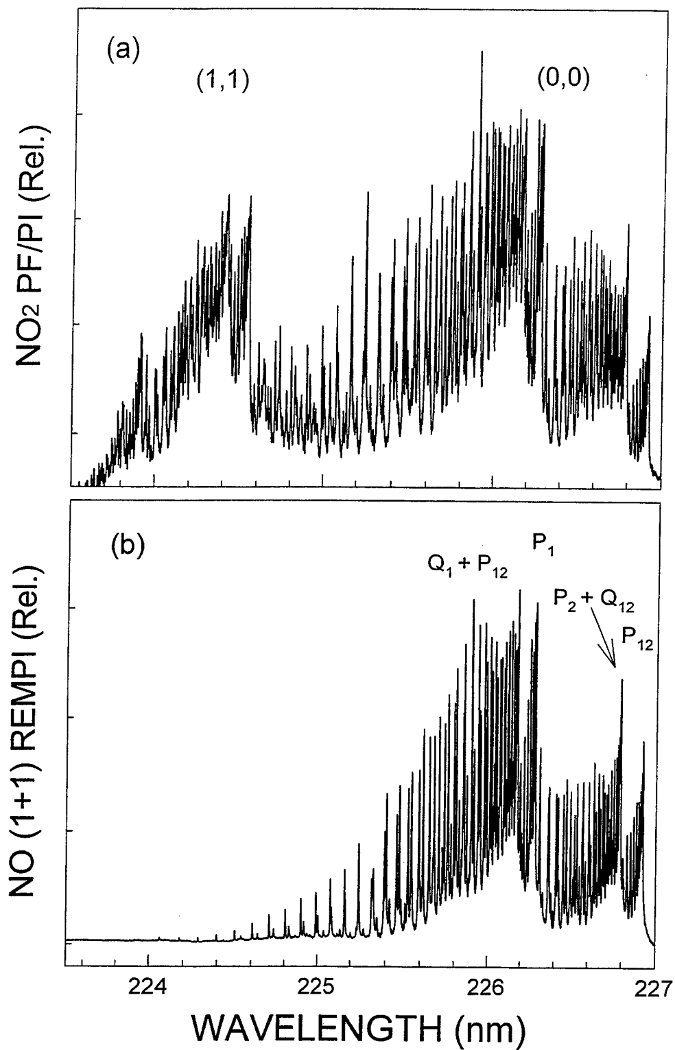
Figure 2. (a) PF/PI spectrum of NO 2 and (b) (1+1) REMPI spectrum of NO in the region of 223–227 nm.
