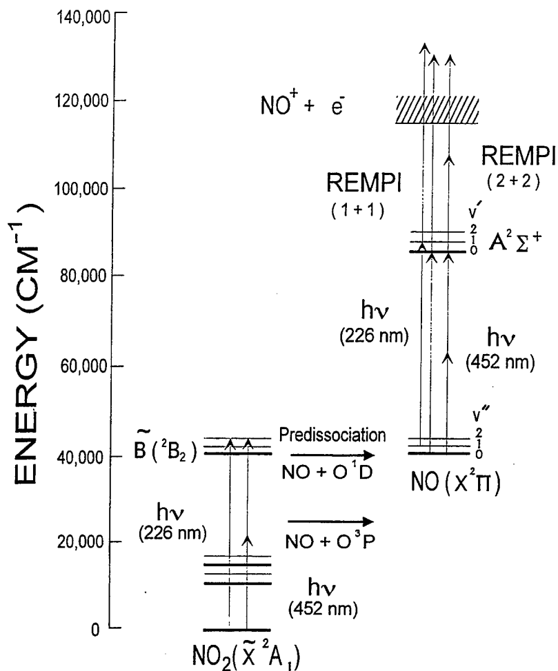
Figure 1. An energy level diagram showing the PF/PI of NO 2 and REMPI of NO at 226 and 452 nm.
